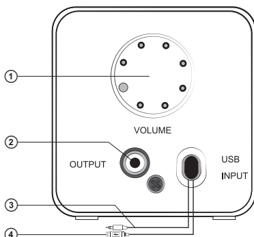
Fig. 1. Rear panel
