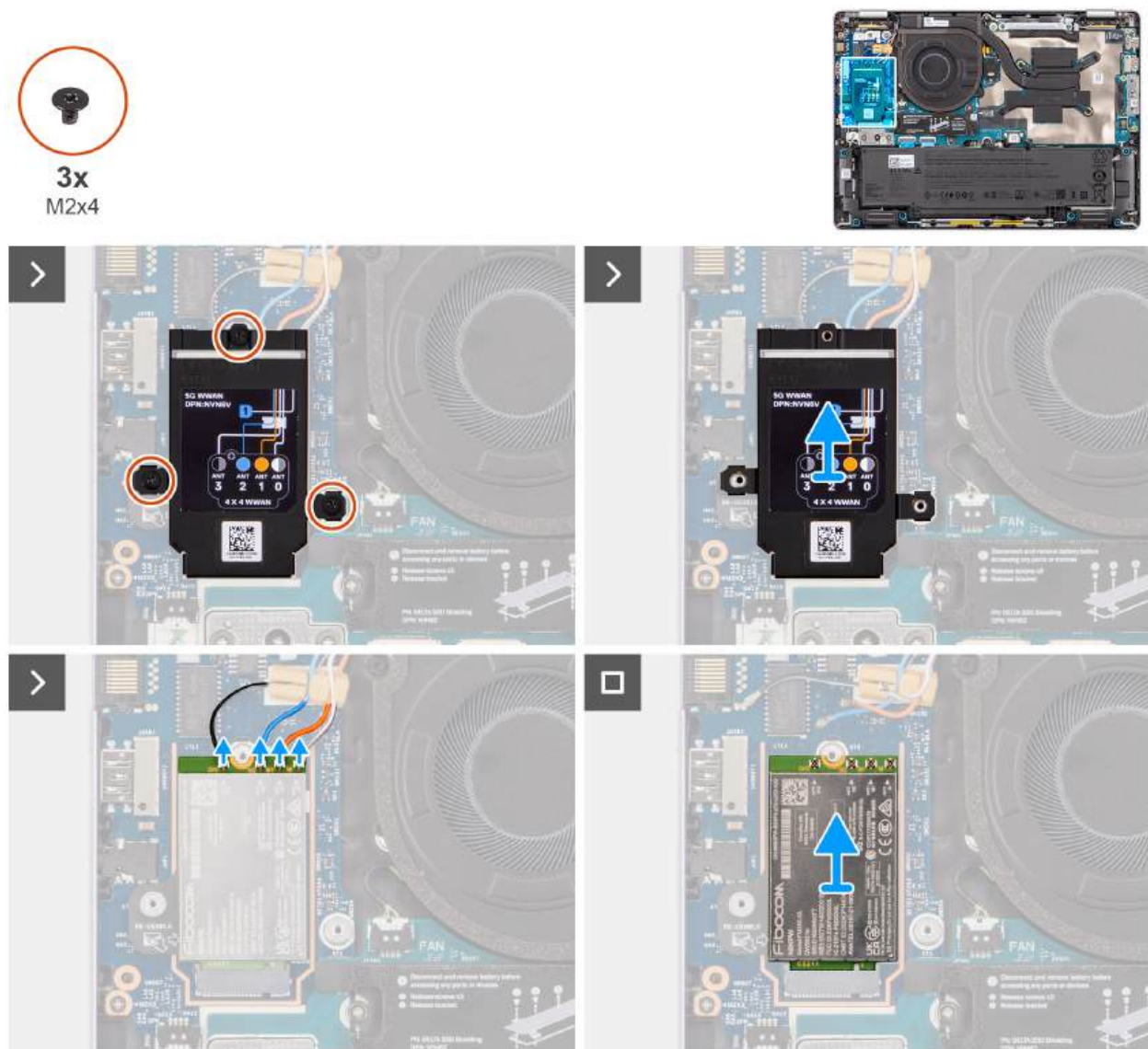
Figure 27. Removing the 5G WWAN card
