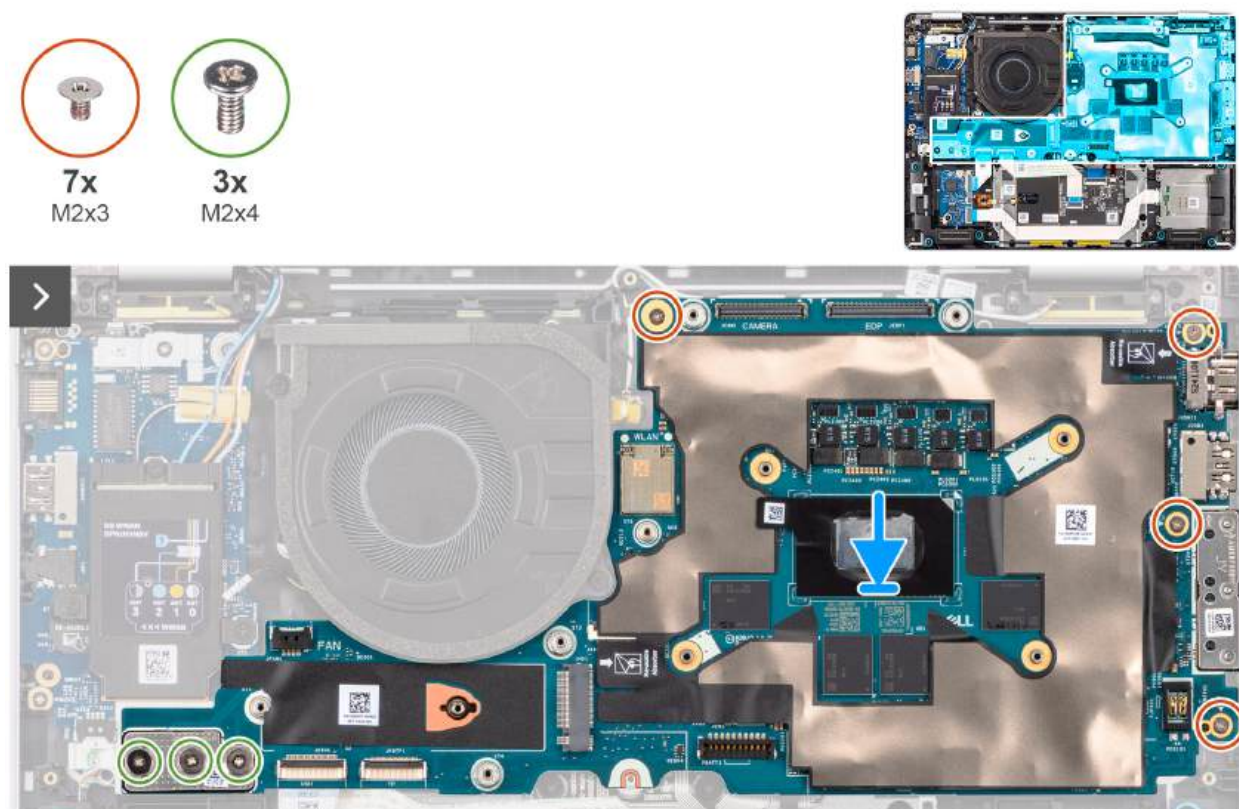
Figure 49. Installing the system board
