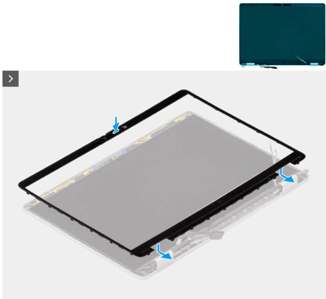
Figure 70. Installing the display bezel
