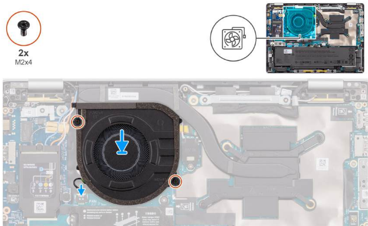
Figure 39. Installing the fan
