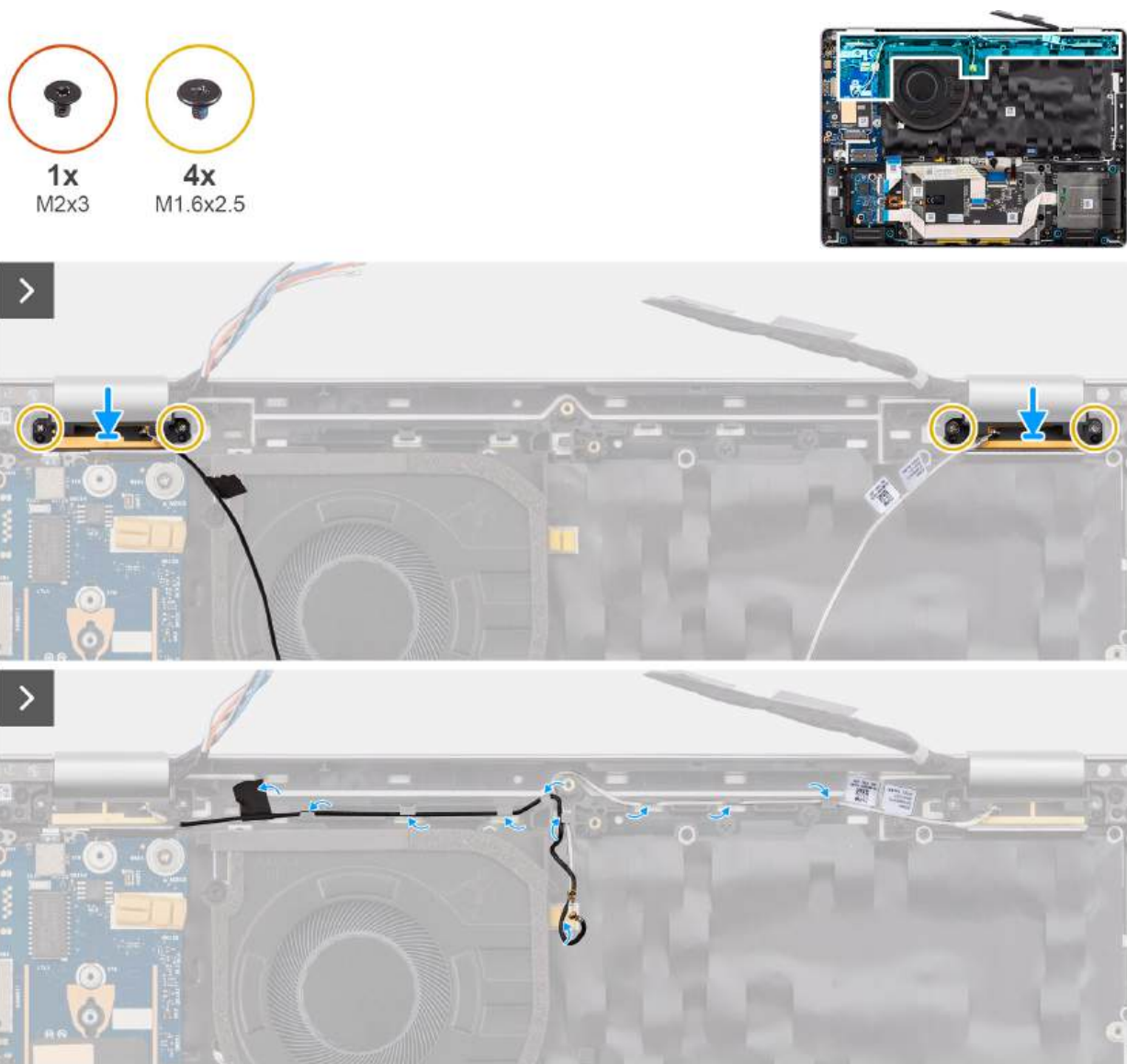
Figure 53. Installing the WLAN antenna modules
