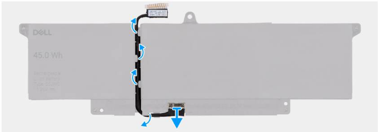
Figure 25. Removing the battery cable
