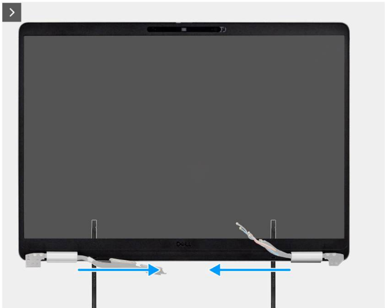
Figure 66. Prying the bezel along the hinges
