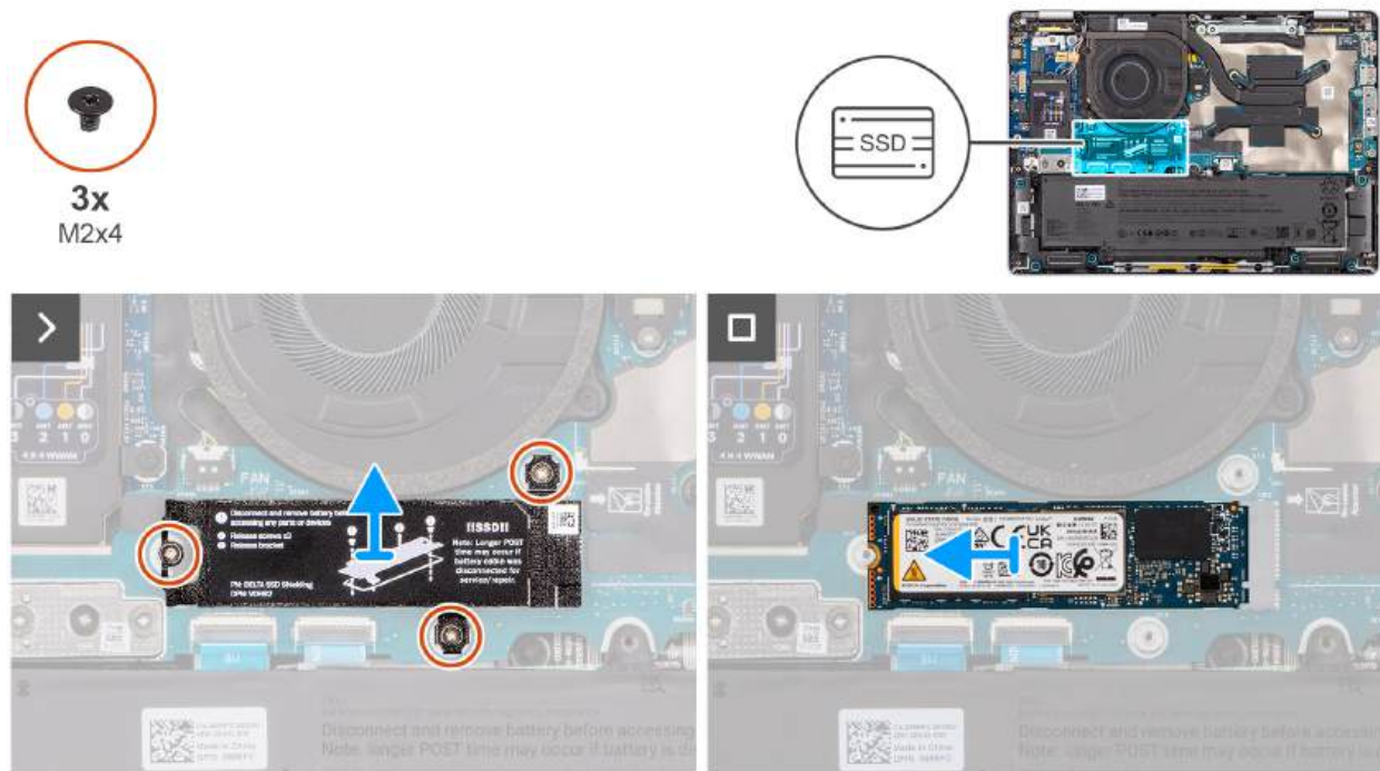
Figure 33. Removing the M.2 2280 SSD
