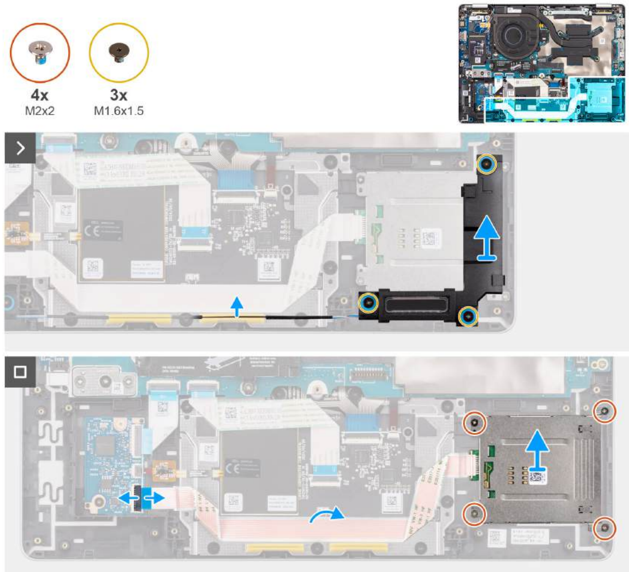
Figure 44. Removing the smart card reader
