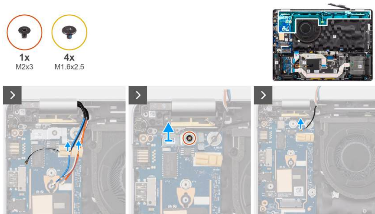
Figure 51. Removing the WLAN antenna modules
