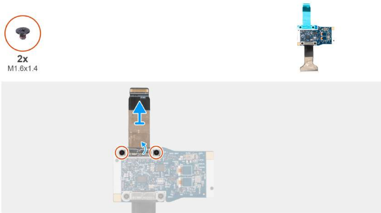
Figure 91. Removing the middle-board cable
