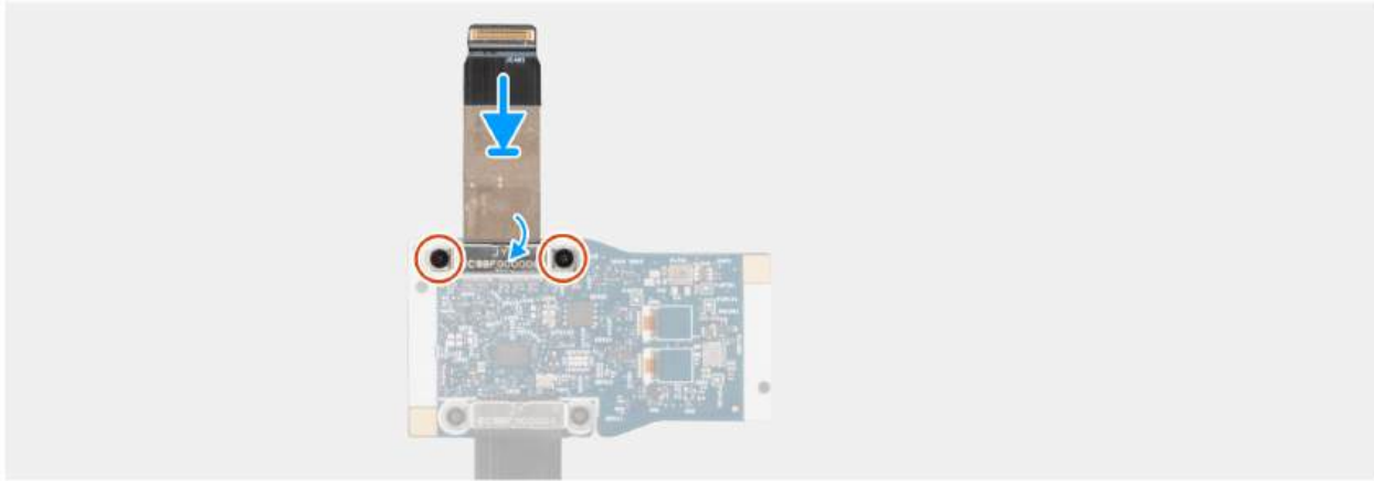
Figure 92. Installing the middle-board cable
