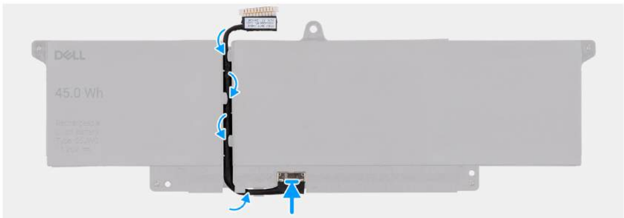
Figure 26. Replacing the battery cable
