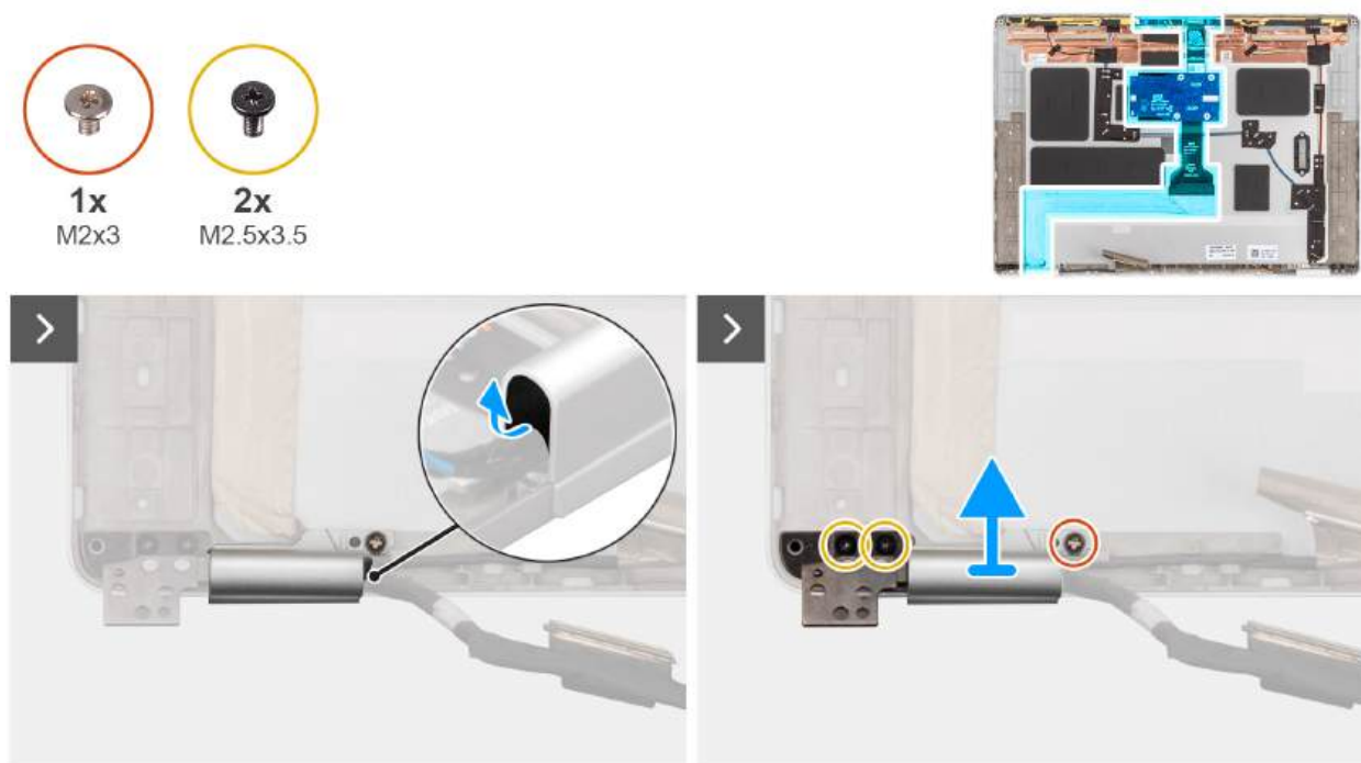
Figure 85. Removing the display cable for RGB/IR camera
