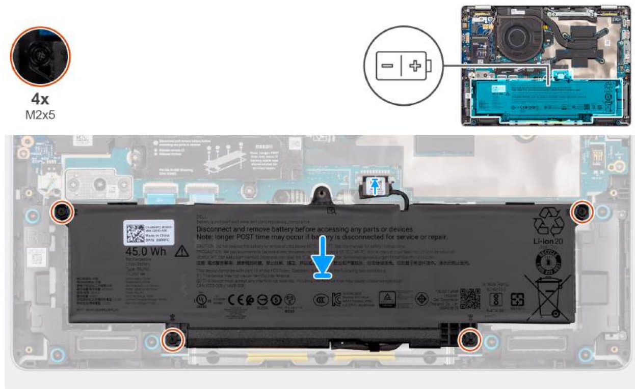
Figure 24. Installing the battery
