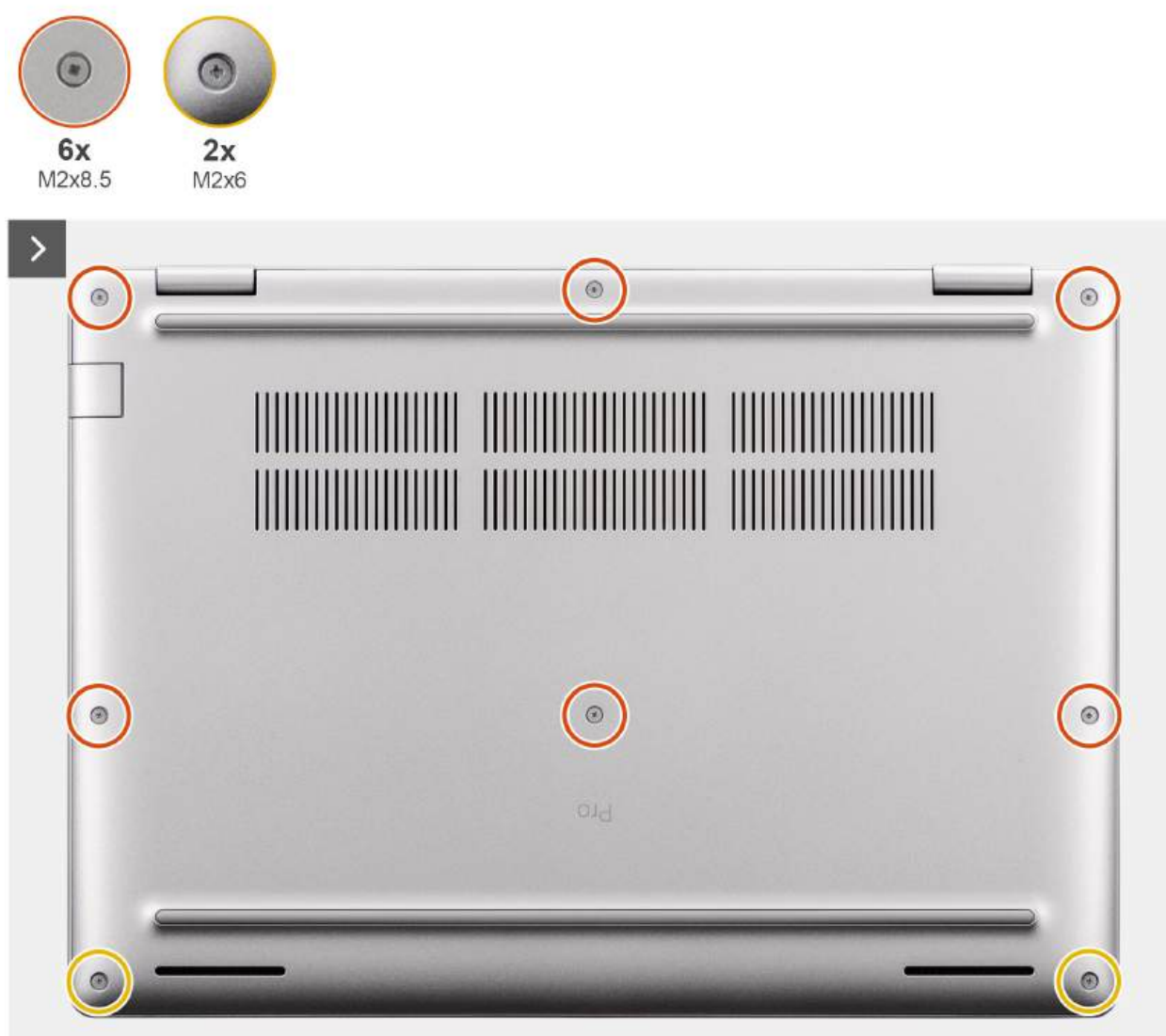
Figure 17. Removing the base cover
