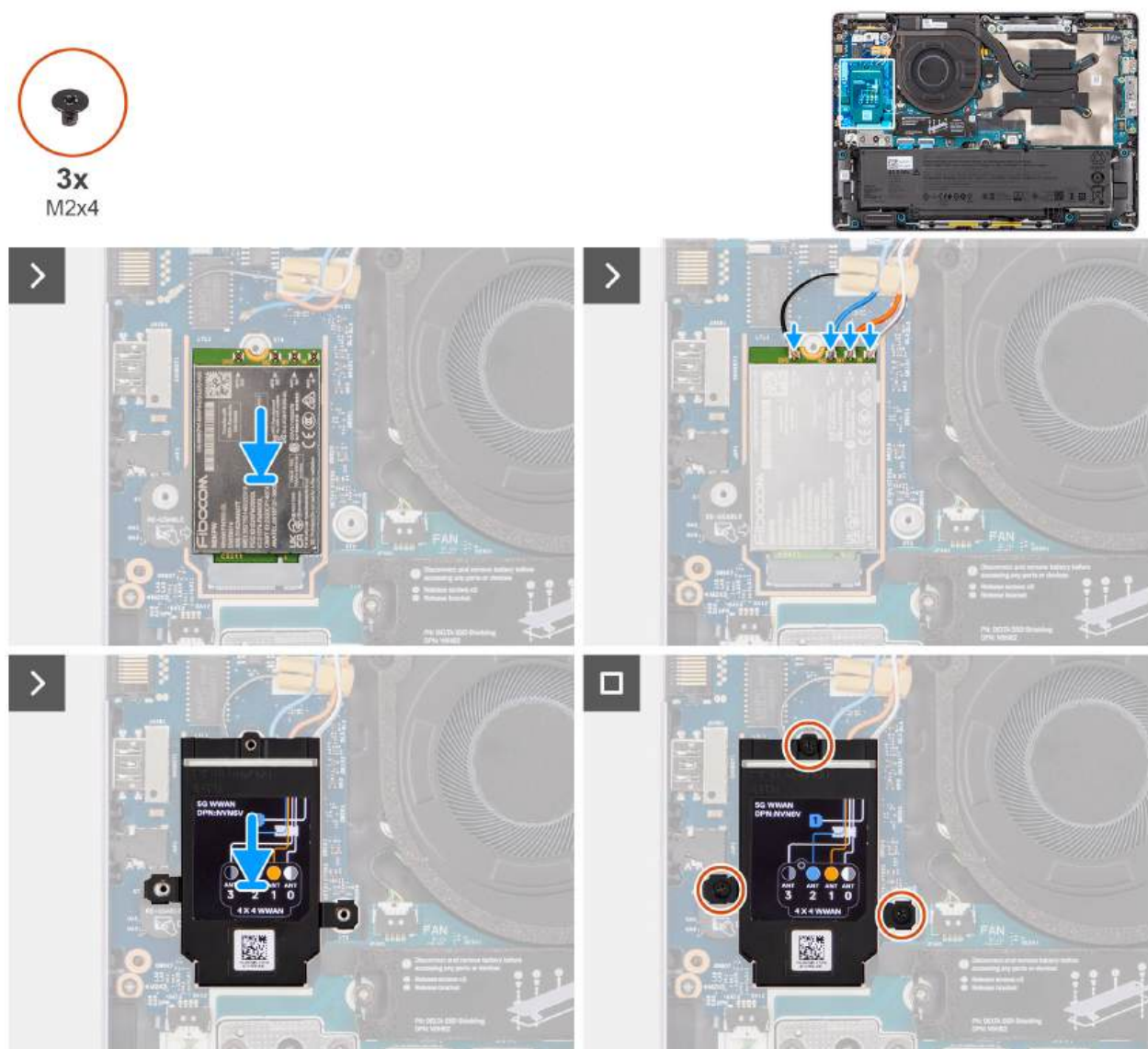
Figure 28. Installing the 5G WWAN card
