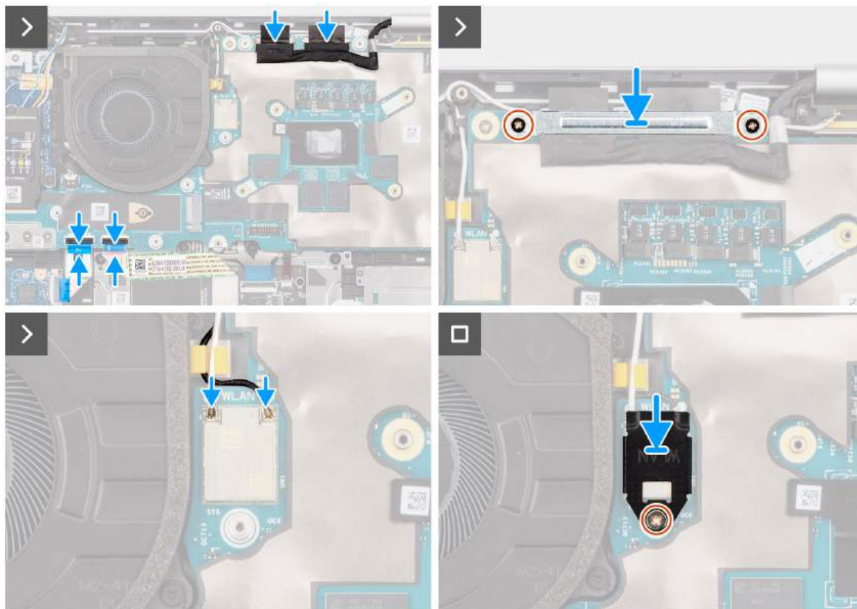
Figure 50. Installing the system board
