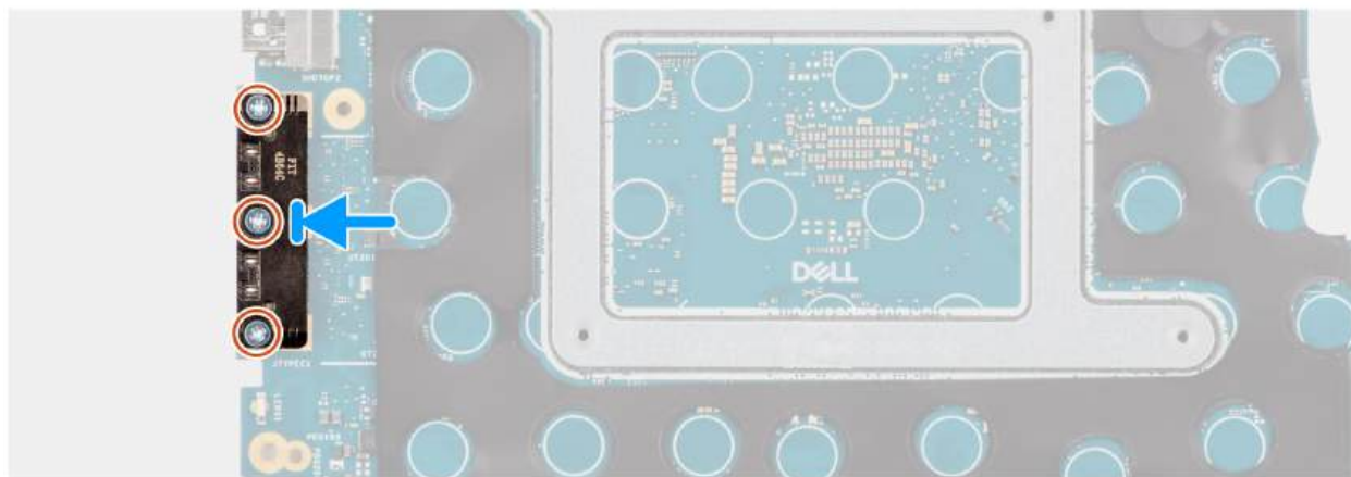
Figure 56. Installing the USB Type-C connector module
