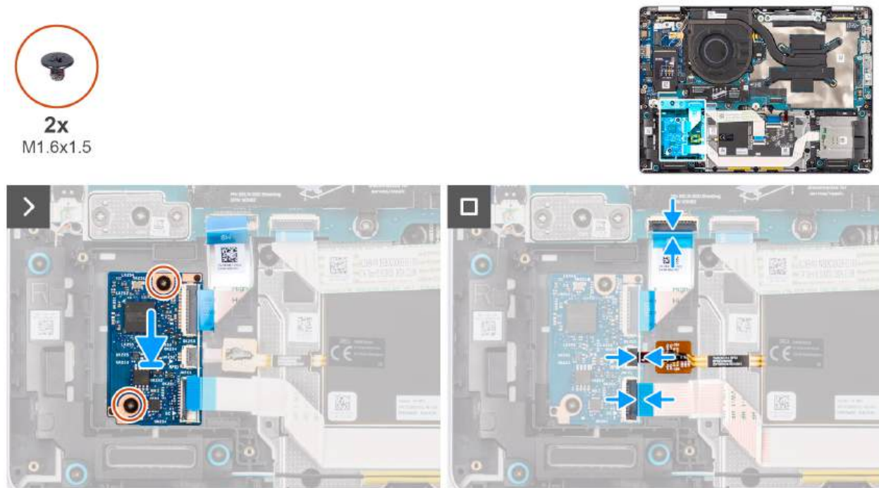
Figure 43. Installing the USH board
