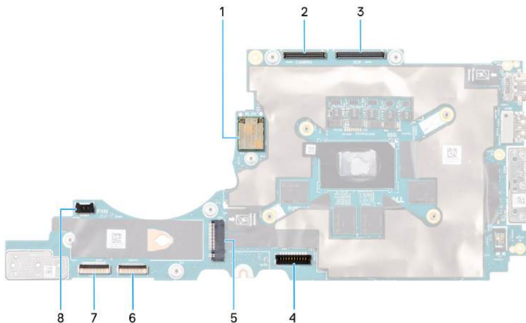
Figure 48. System board slots and connectors
