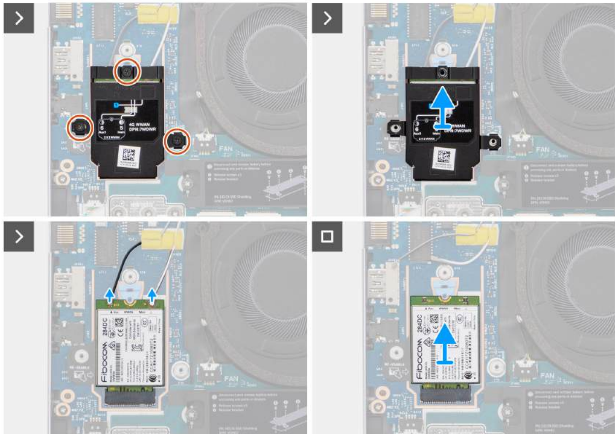
Figure 29. Removing the 4G WWAN card
