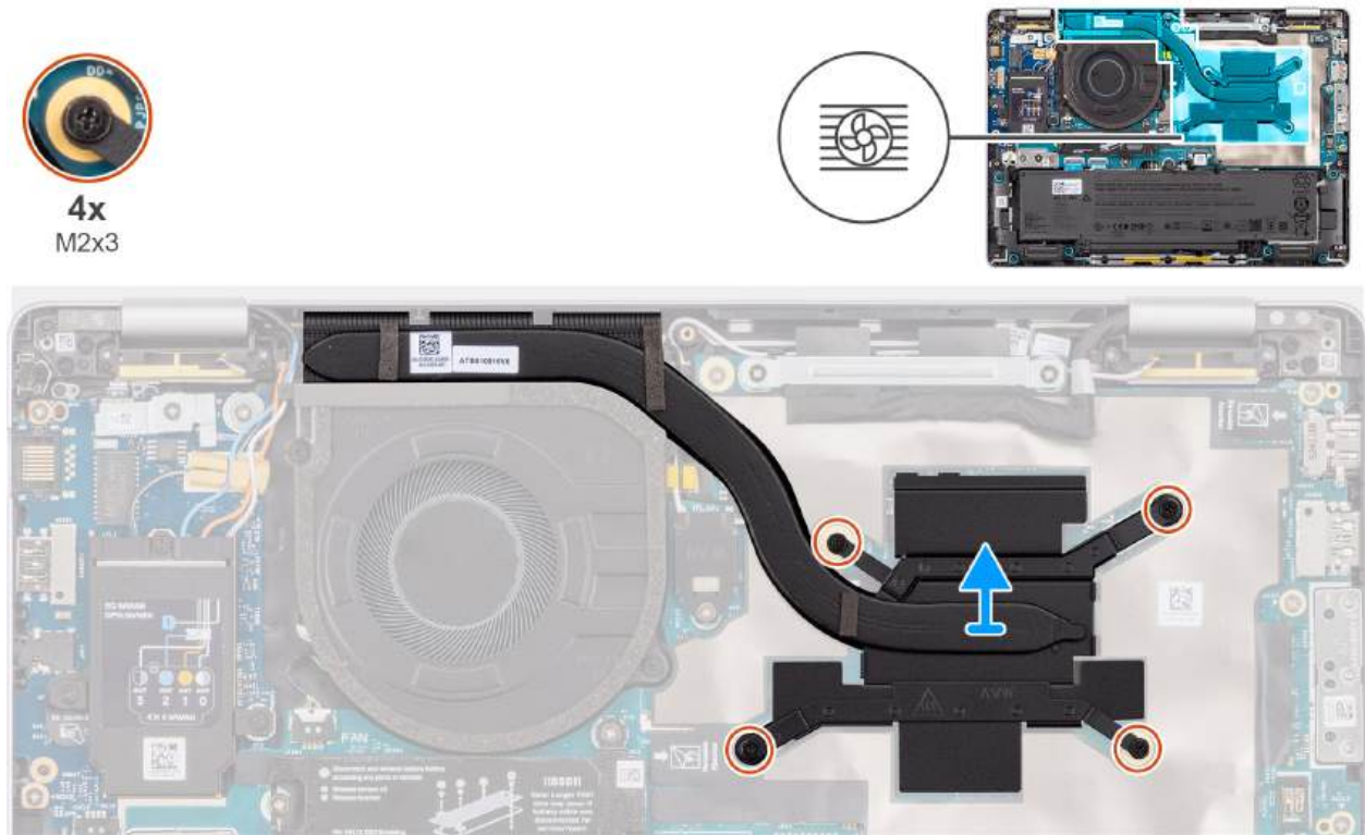
Figure 40. Removing the heat sink
