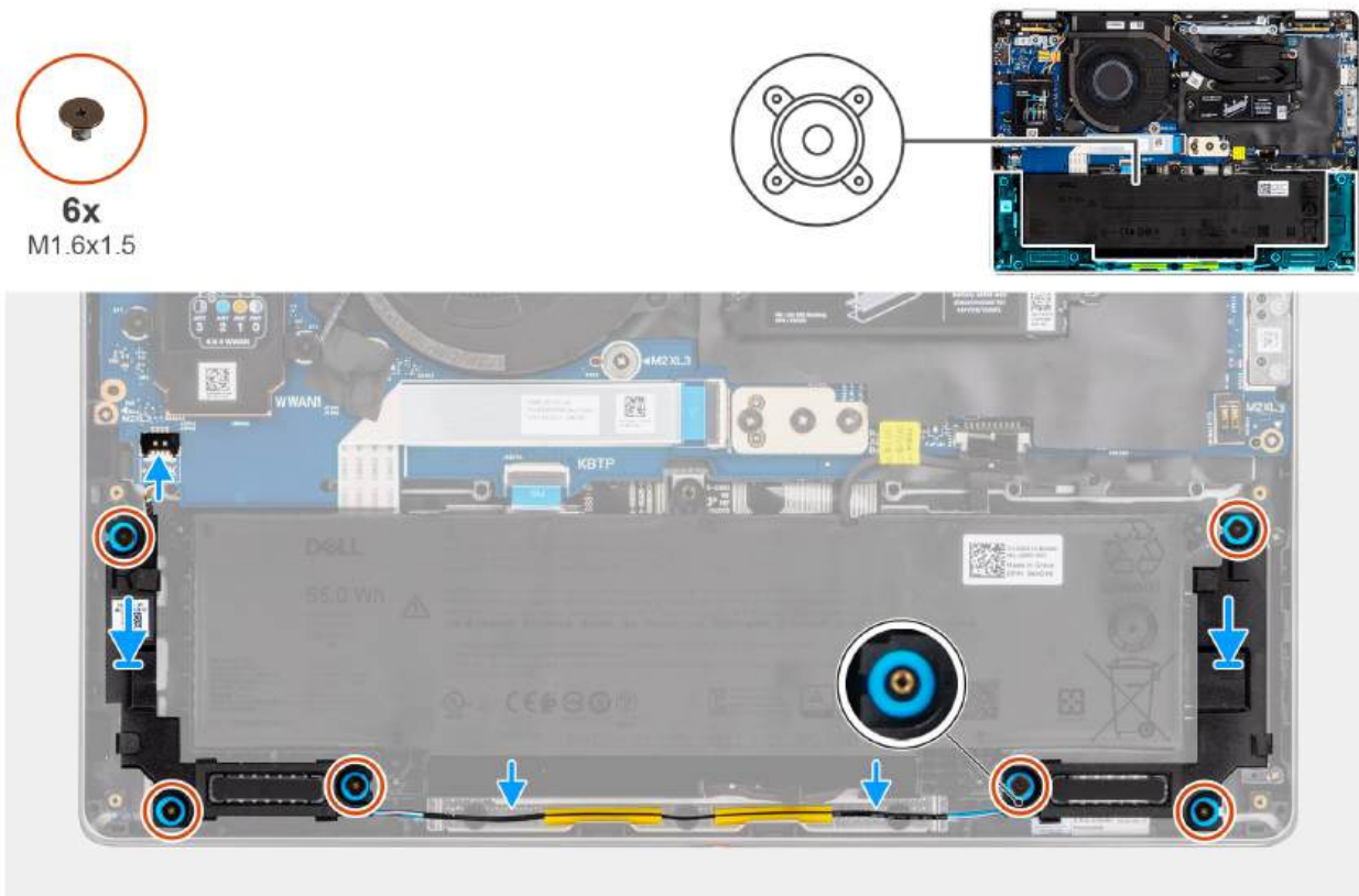
Figure 36. Installing the speakers
