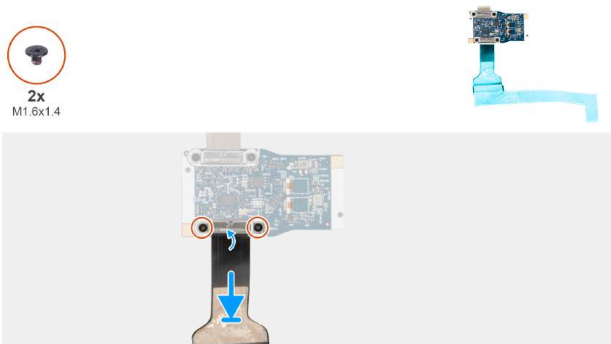
Figure 90. Installing the display cable for MIPI camera to middle board
