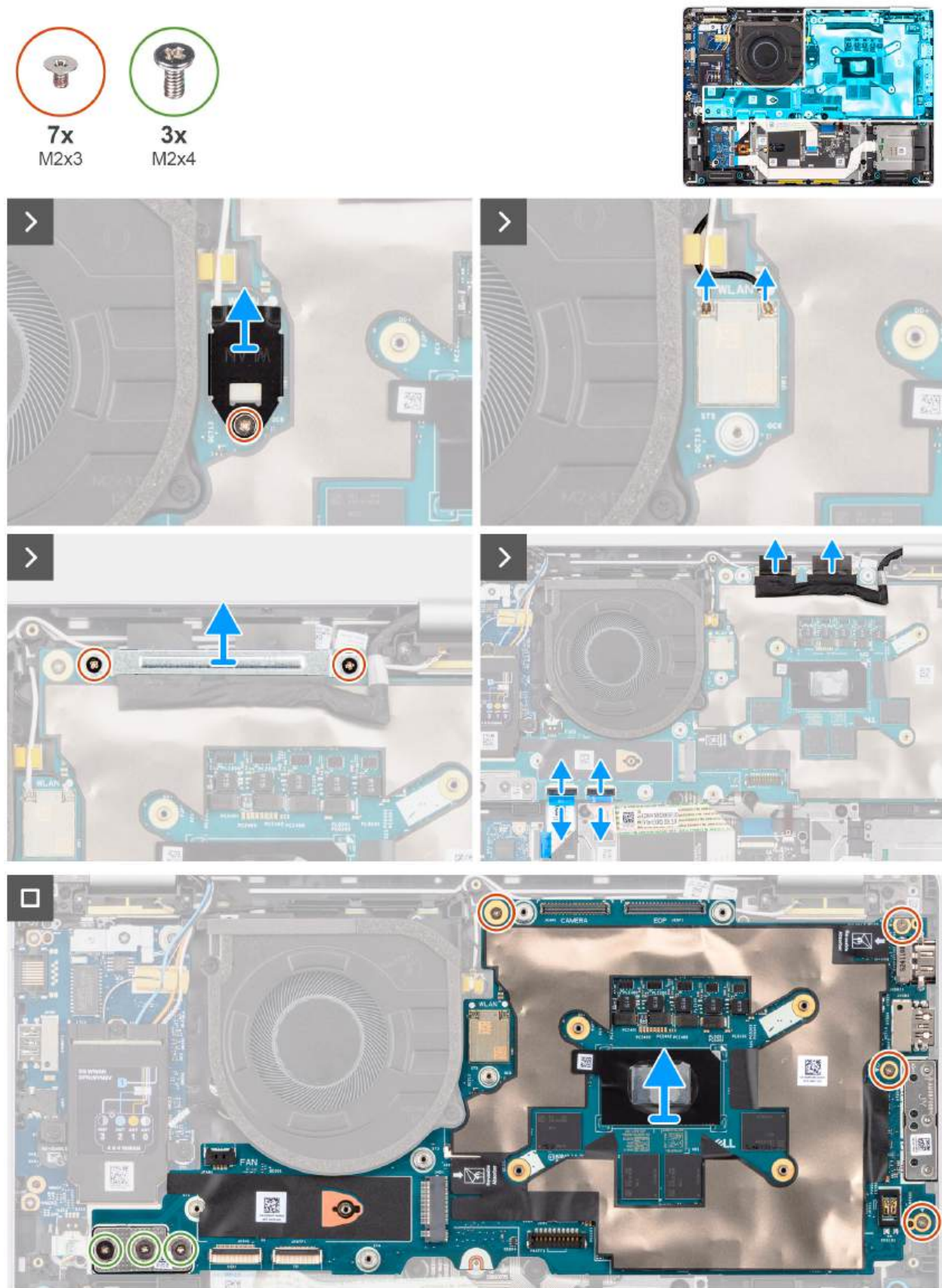
Figure 47. Removing the system board
