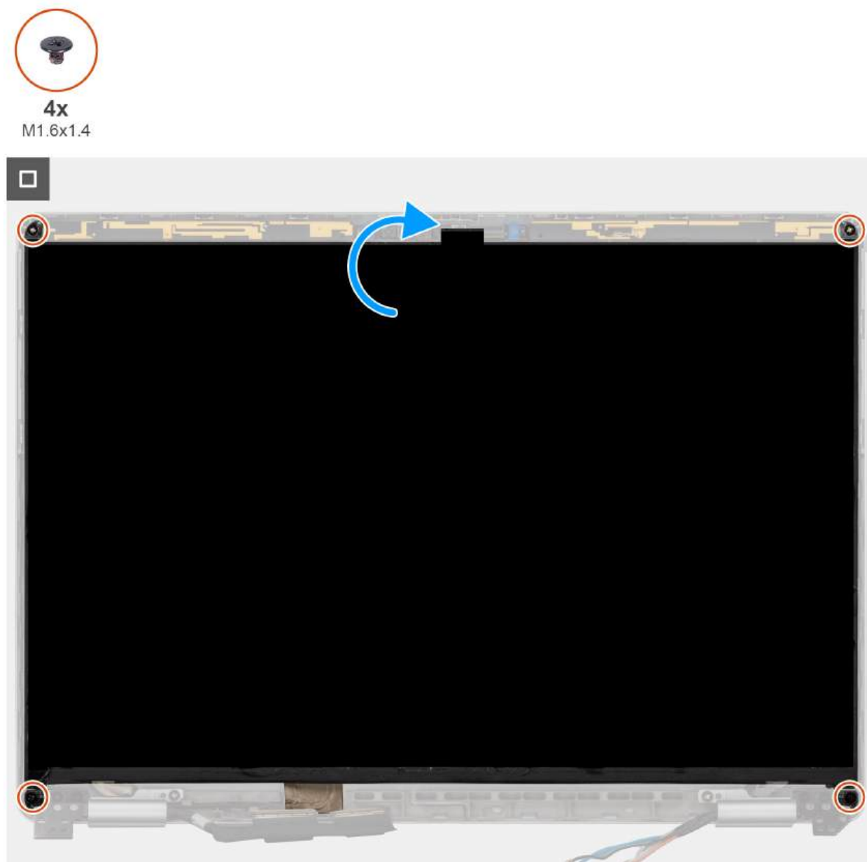
Figure 76. Installing the display panel
