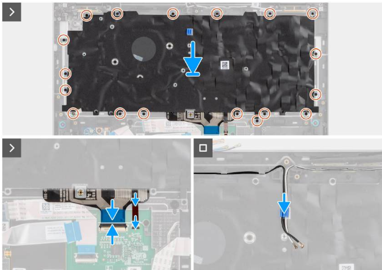
Figure 100. Installing the keyboard
