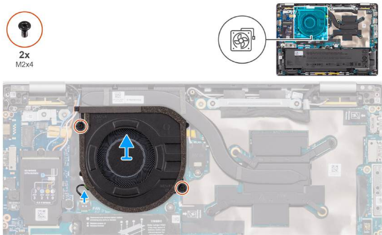
Figure 38. Removing the fan
