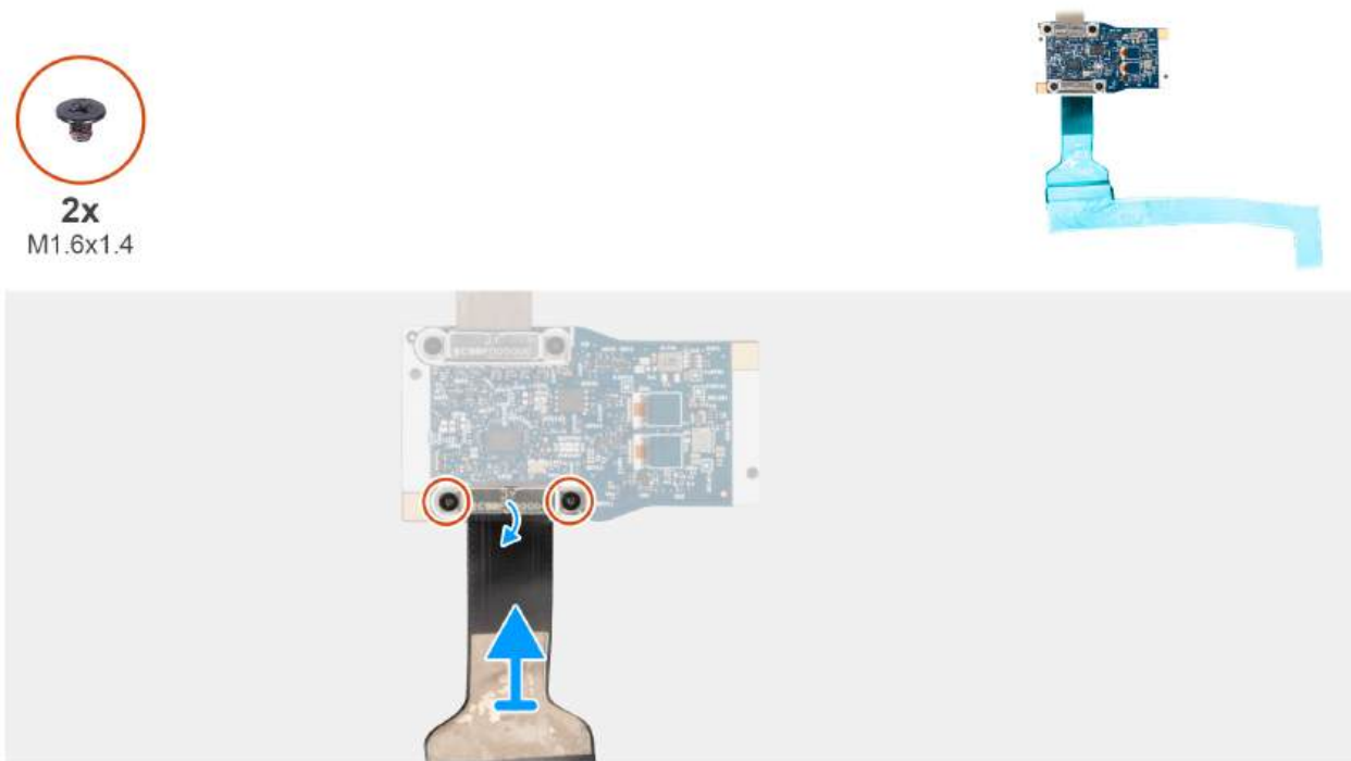
Figure 89. Removing the display cable for MIPI camera from middle board
