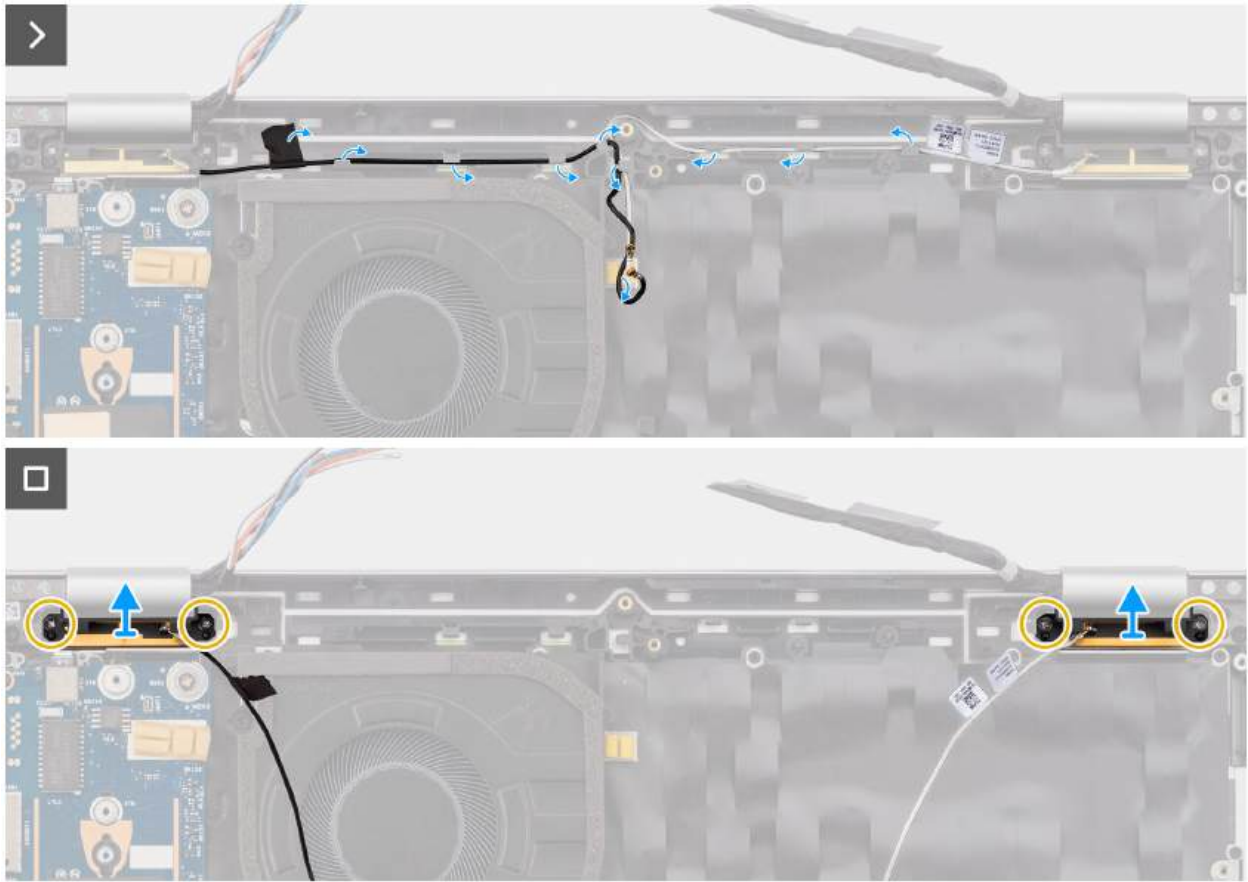
Figure 52. Removing the WLAN antenna modules
