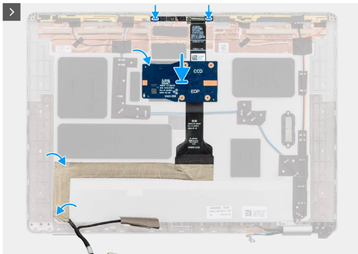
Figure 87. Installing the display cable for RGB/IR camera
