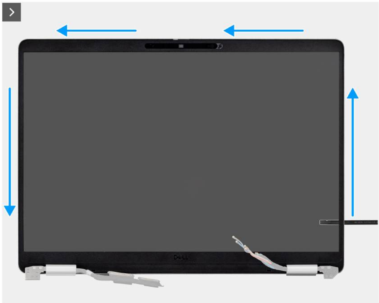
Figure 68. Prying the bezel along the sides
