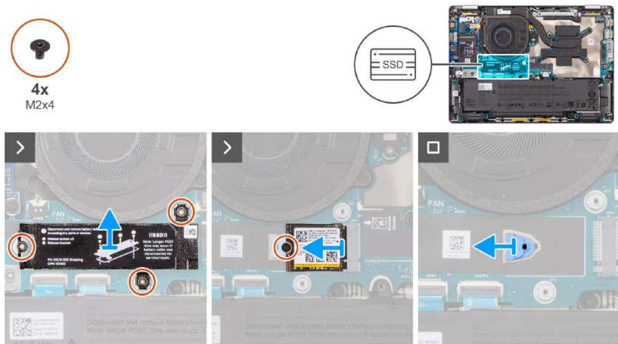
Figure 31. Removing the M.2 2230 SSD
