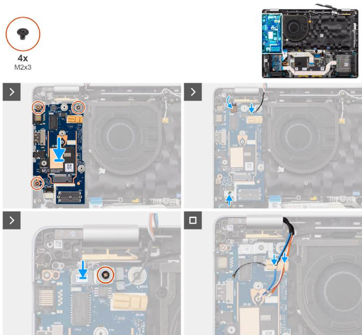
Figure 58. Installing the I/O board
