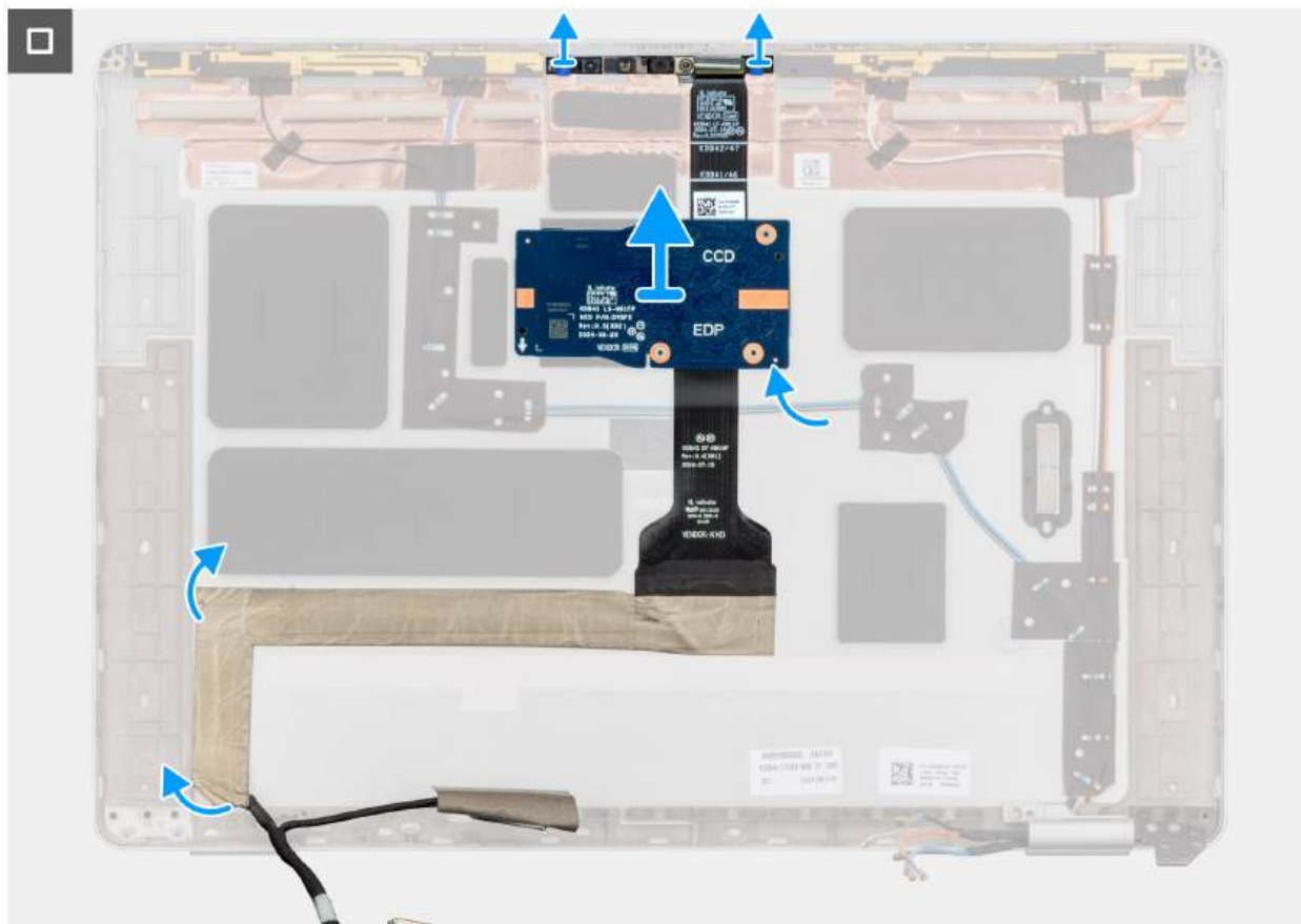
Figure 86. Removing the display cable for RGB/IR camera
