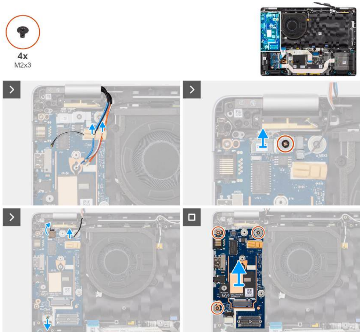
Figure 57. Removing the I/O board
