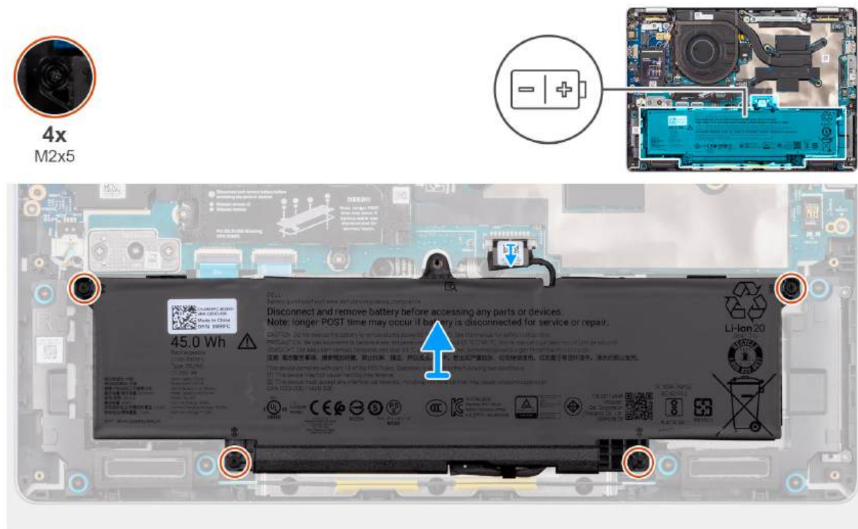
Figure 23. Removing the battery
