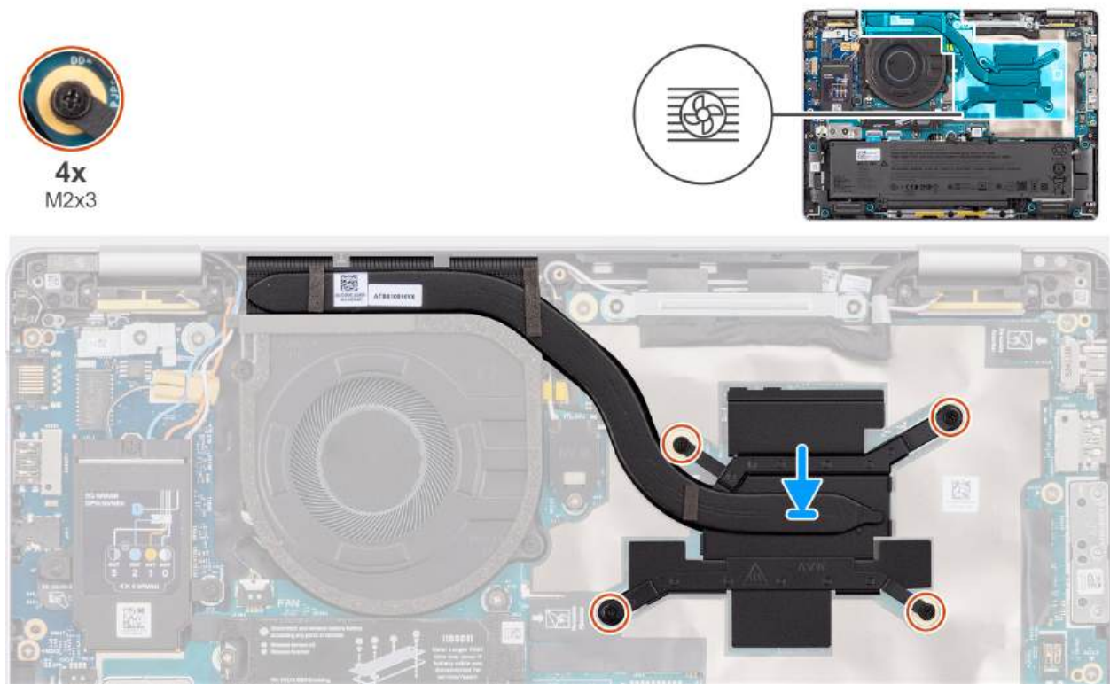
Figure 41. Installing the heat sink
