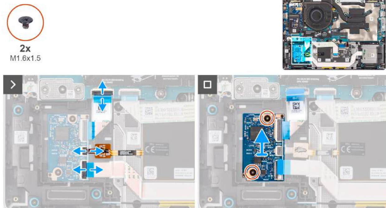
Figure 42. Removing the USH board
