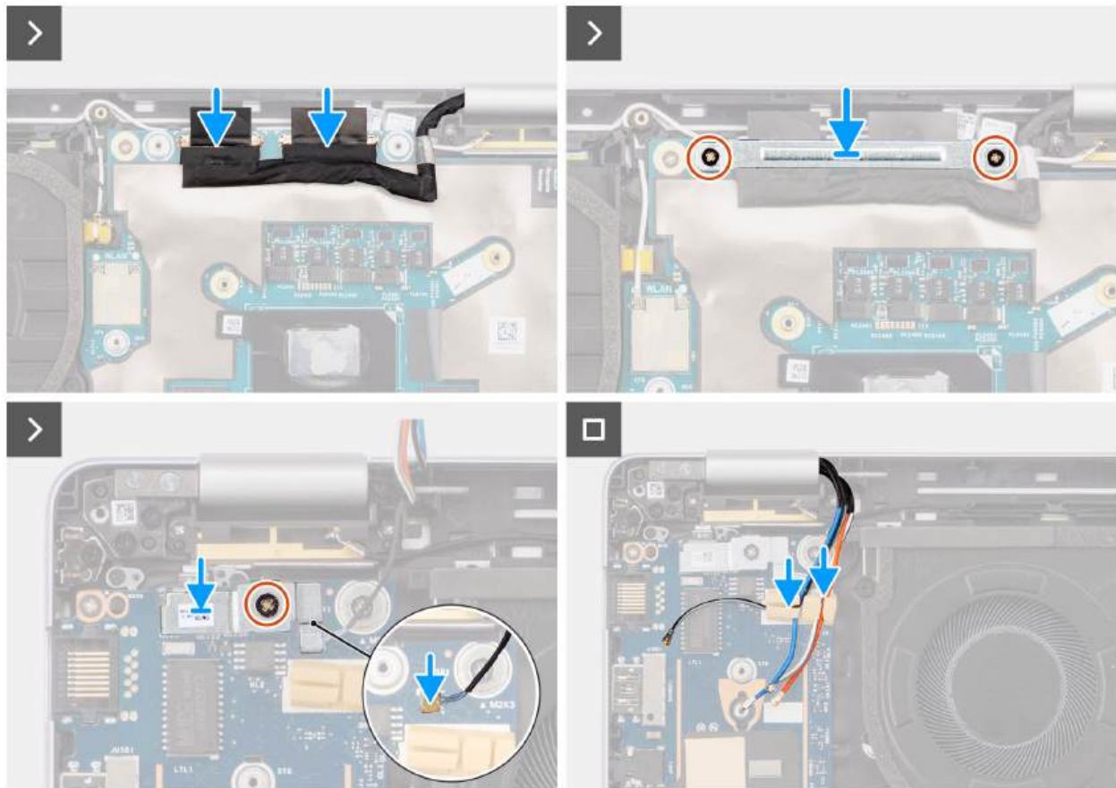
Figure 64. Installing the display assembly
