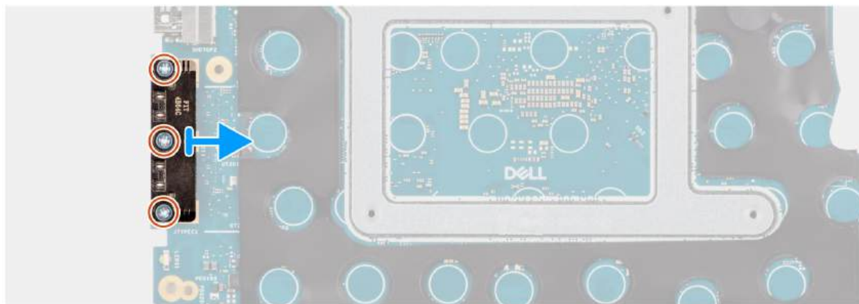
Figure 55. Removing the USB Type-C connector module
