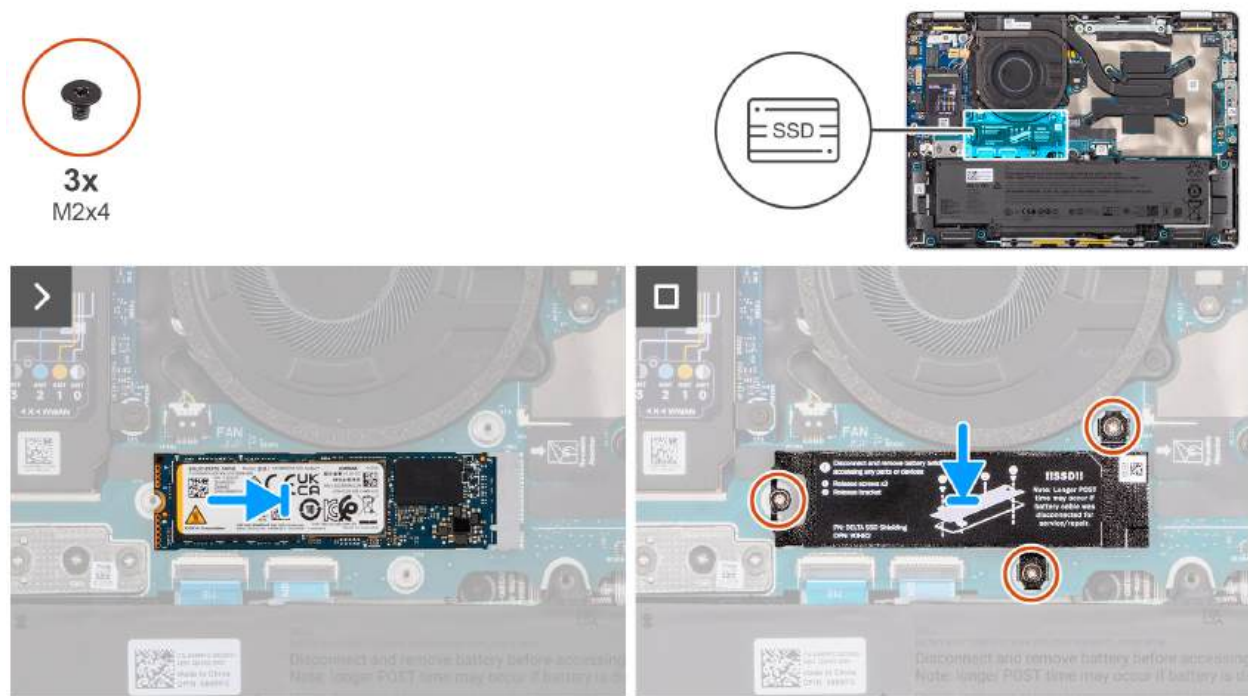
Figure 34. Installing the M.2 2280 SSD
