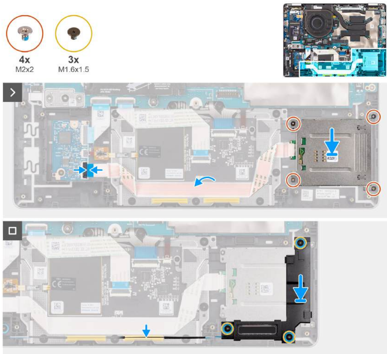
Figure 45. Installing the smart card reader
