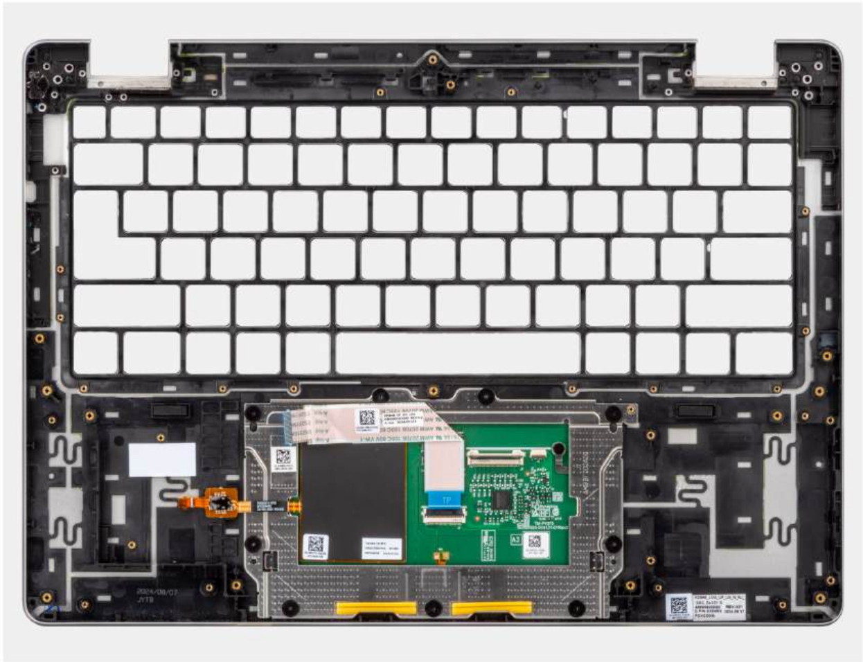
Figure 101. Palm-rest assembly
