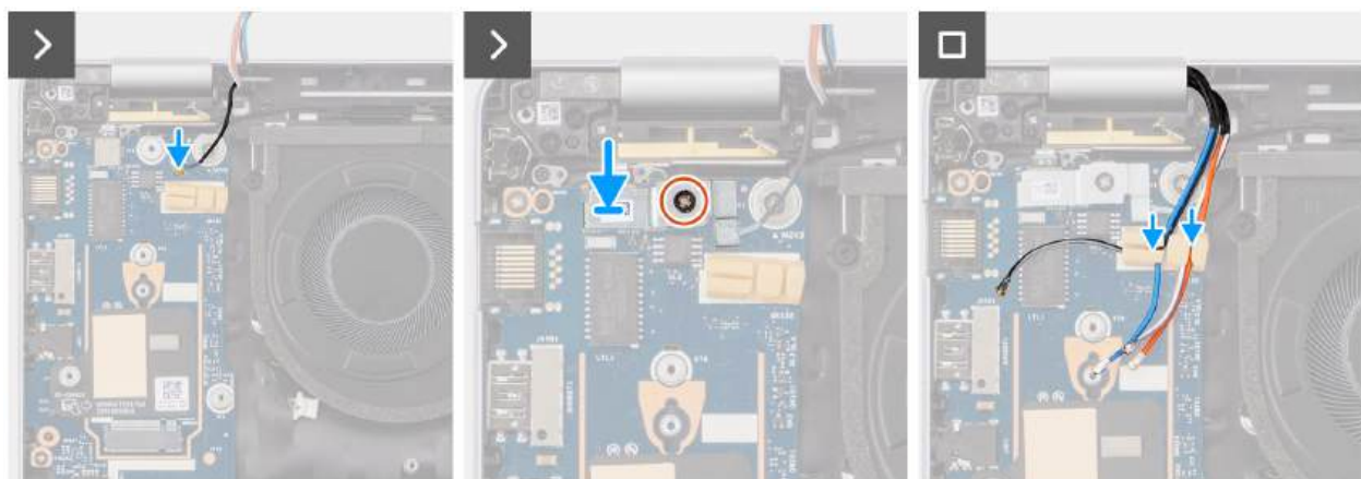
Figure 54. Installing the WLAN antenna modules
