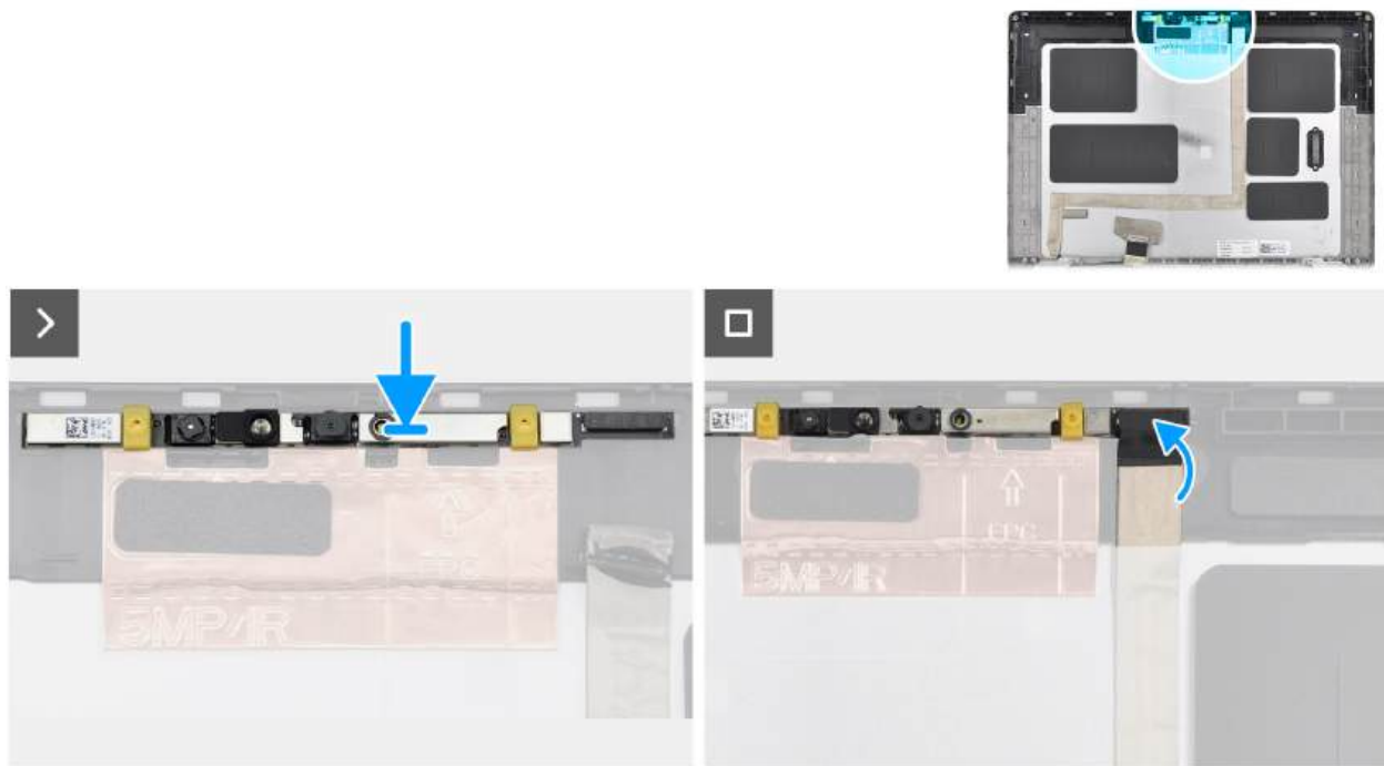
Figure 81. Installing the IR camera
