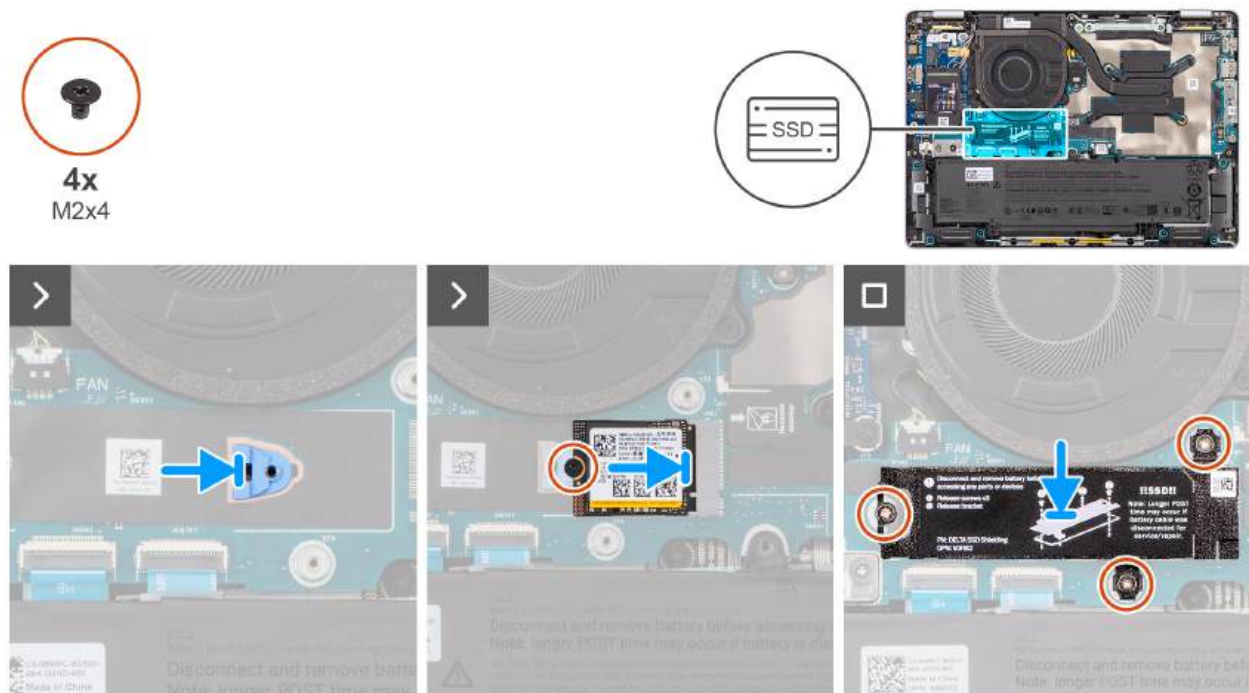
Figure 32. Installing the M.2 2230 SSD
