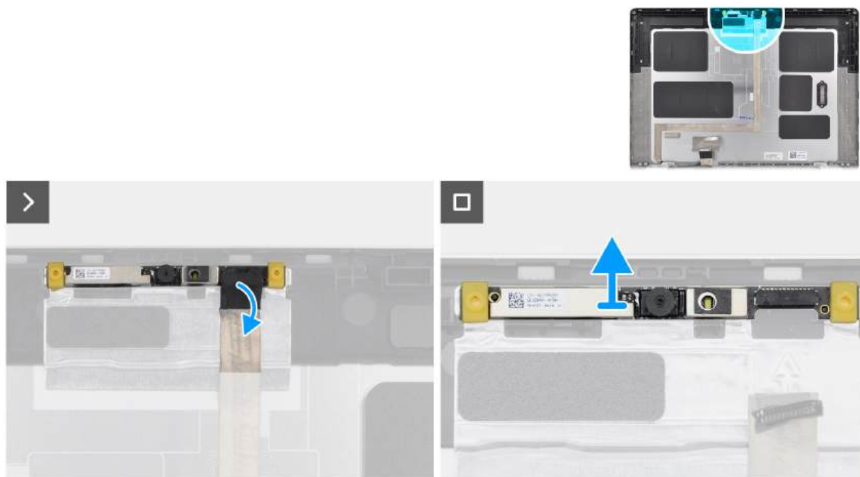
Figure 80. Removing the RGB camera
