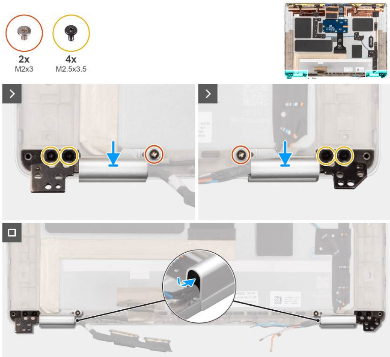
Figure 78. Installing the hinge caps
