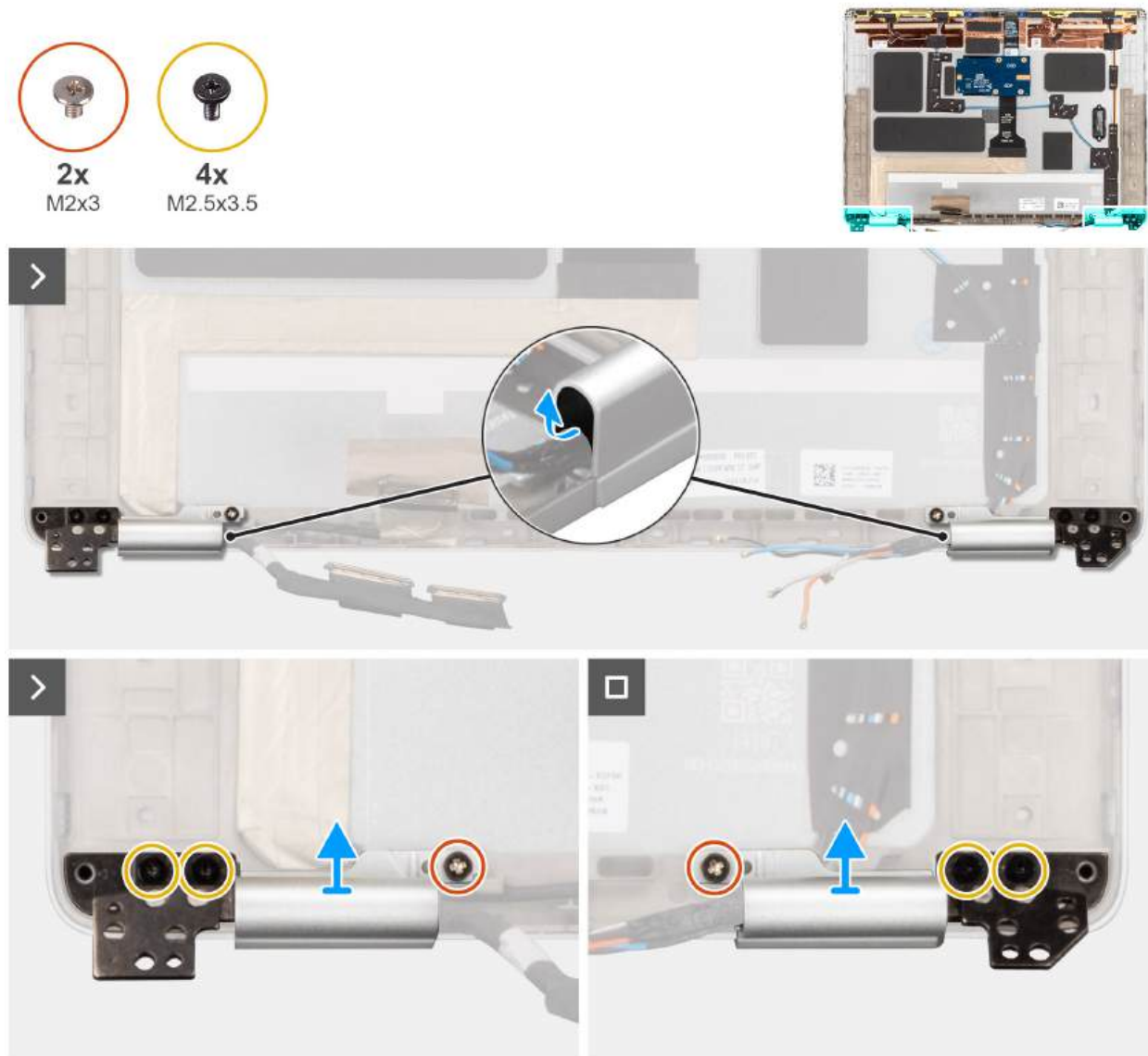
Figure 77. Removing the display hinges
