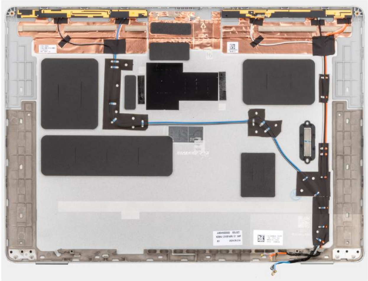
Figure 95. Removing display back-cover and antenna assembly
