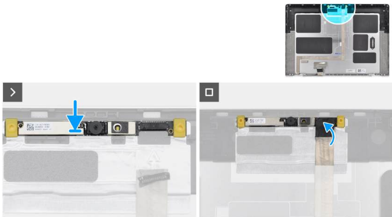
Figure 82. Installing the RGB camera
