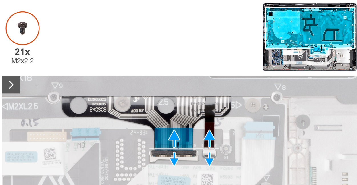
Figure 94. Removing the keyboard
