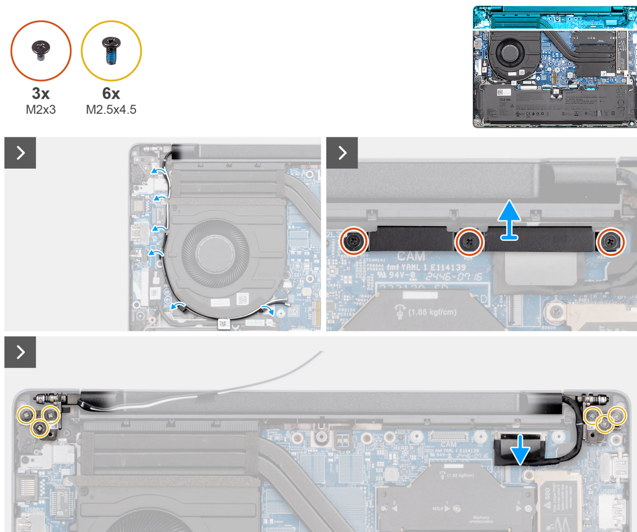
Figure 47. Removing the display assembly
