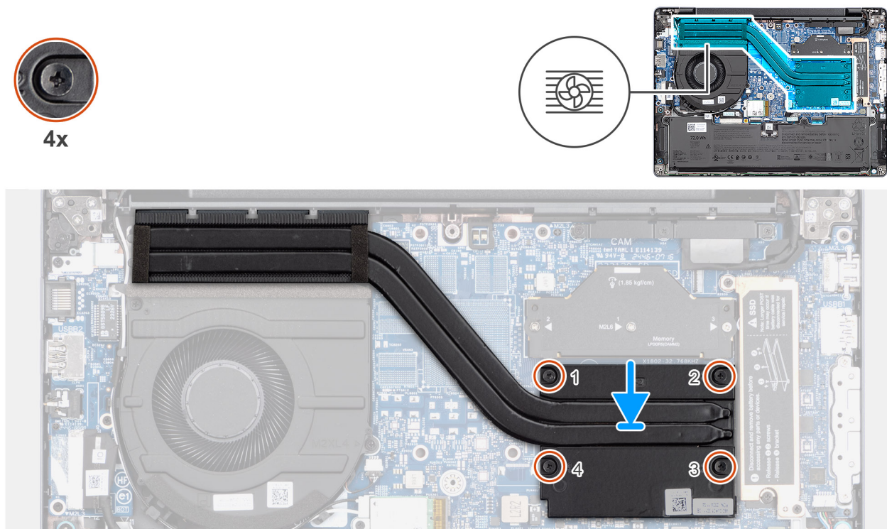
Figure 40. Installing the heat sink
