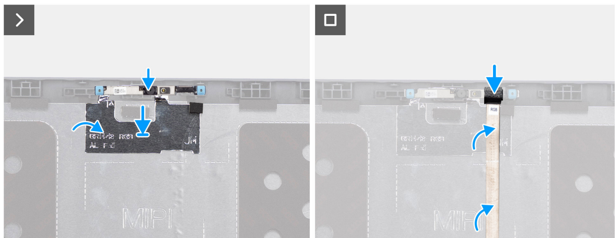
Figure 71. Installing the camera
