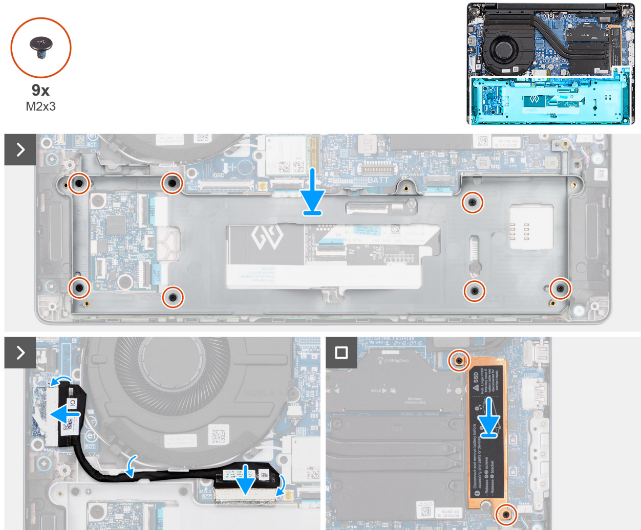
Figure 34. Installing the battery frame
