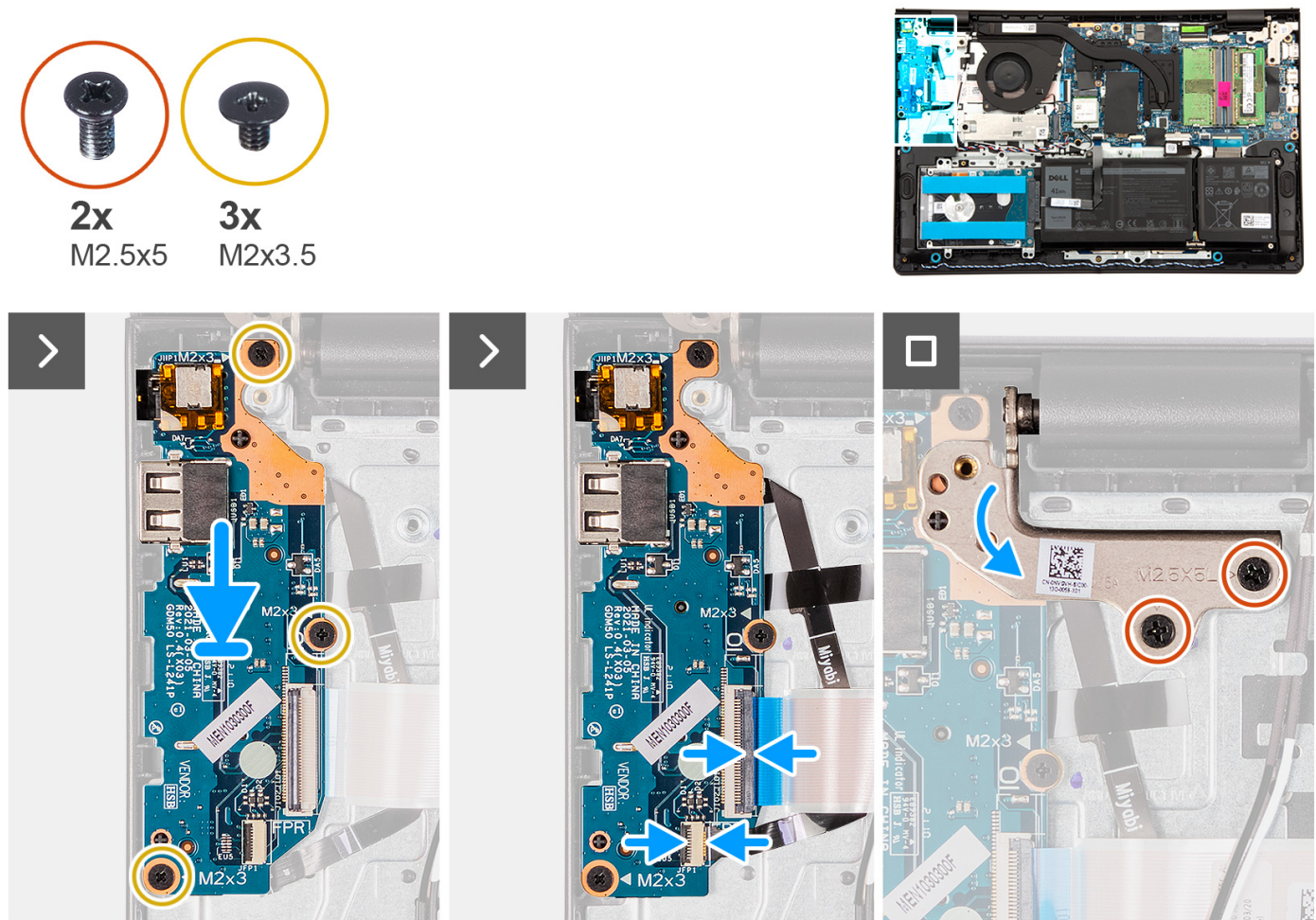
Figure 4. Installing I/O daughter-board
