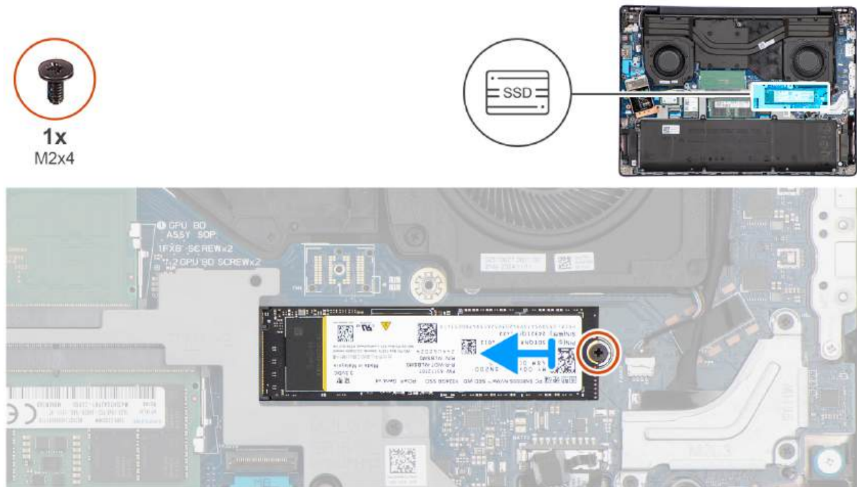
Figure 25. Removing the M.2 2280 solid state drive
