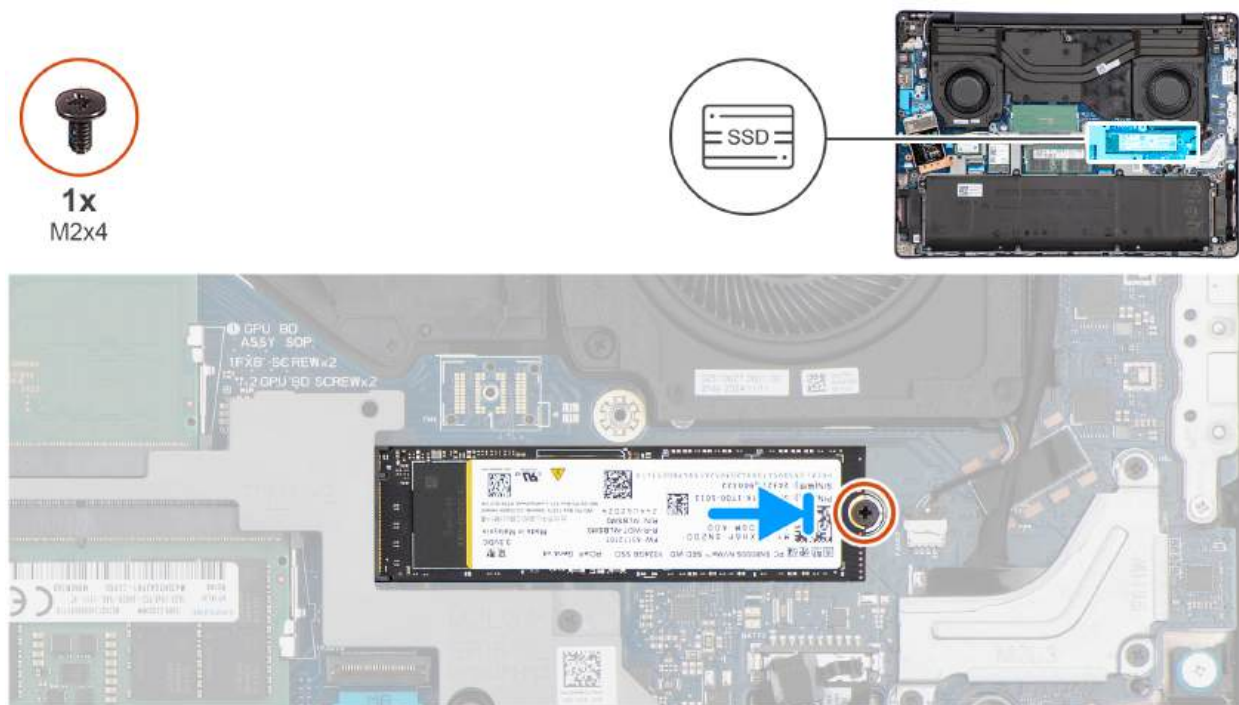
Figure 26. Installing the M.2 2280 solid state drive
