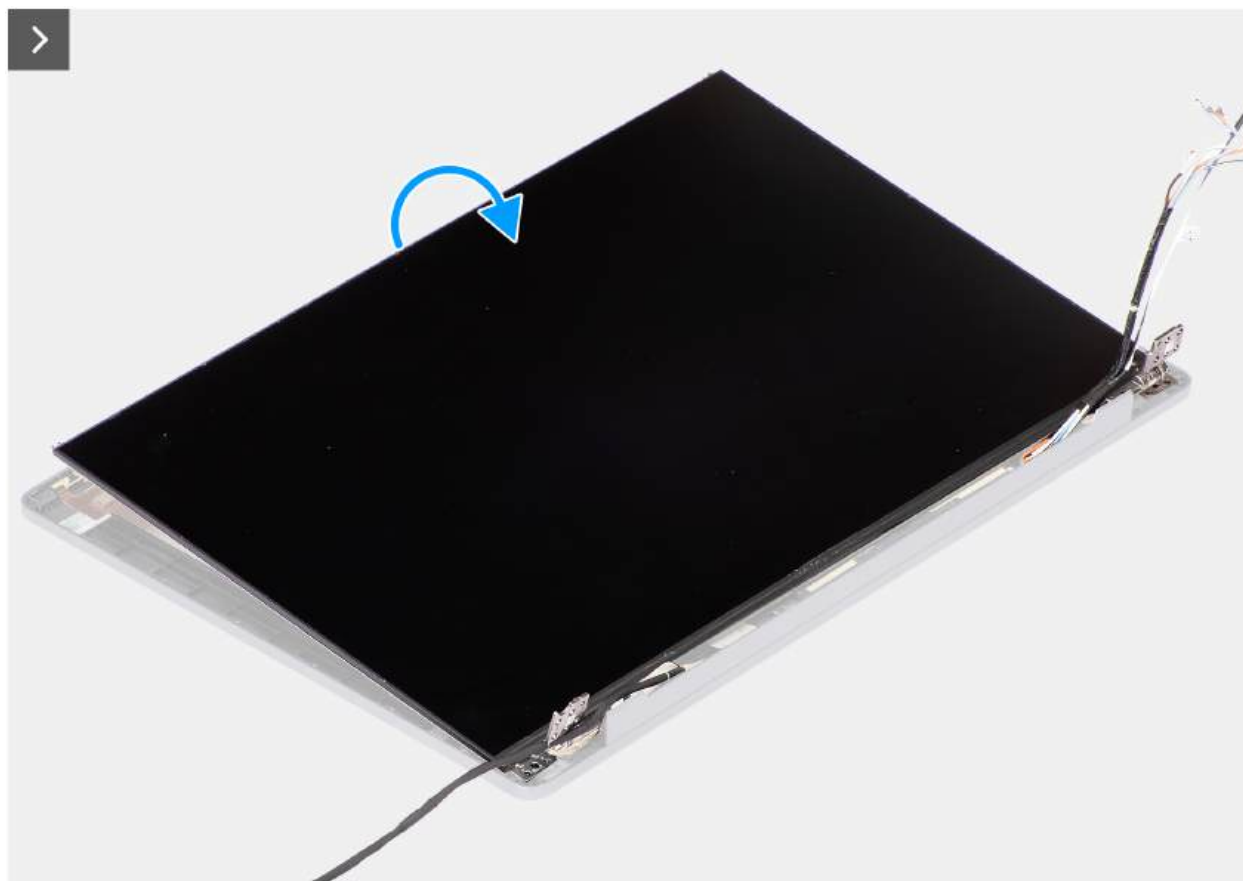
Figure 69. Removing the display panel
