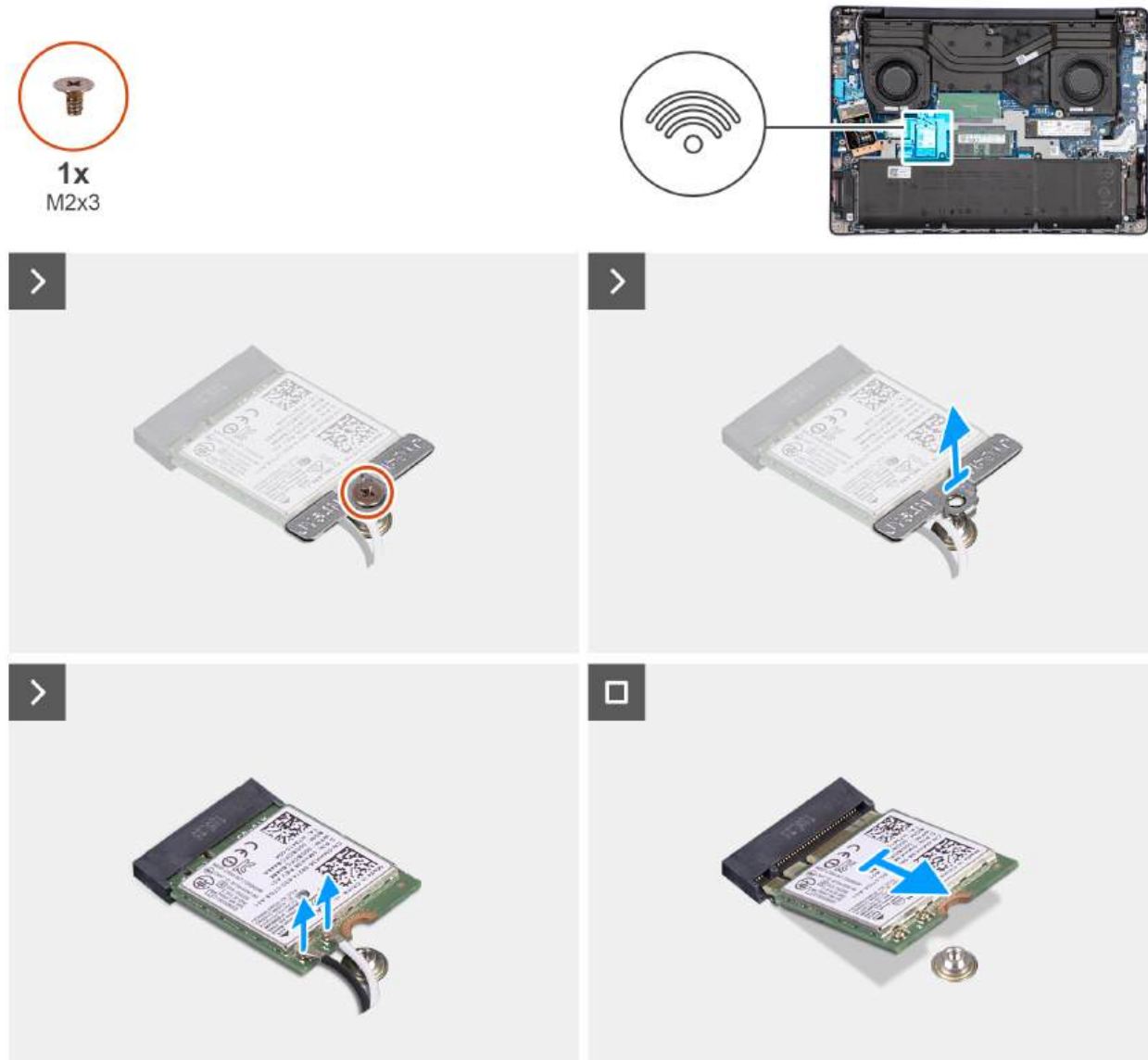
Figure 27. Removing the wireless card
