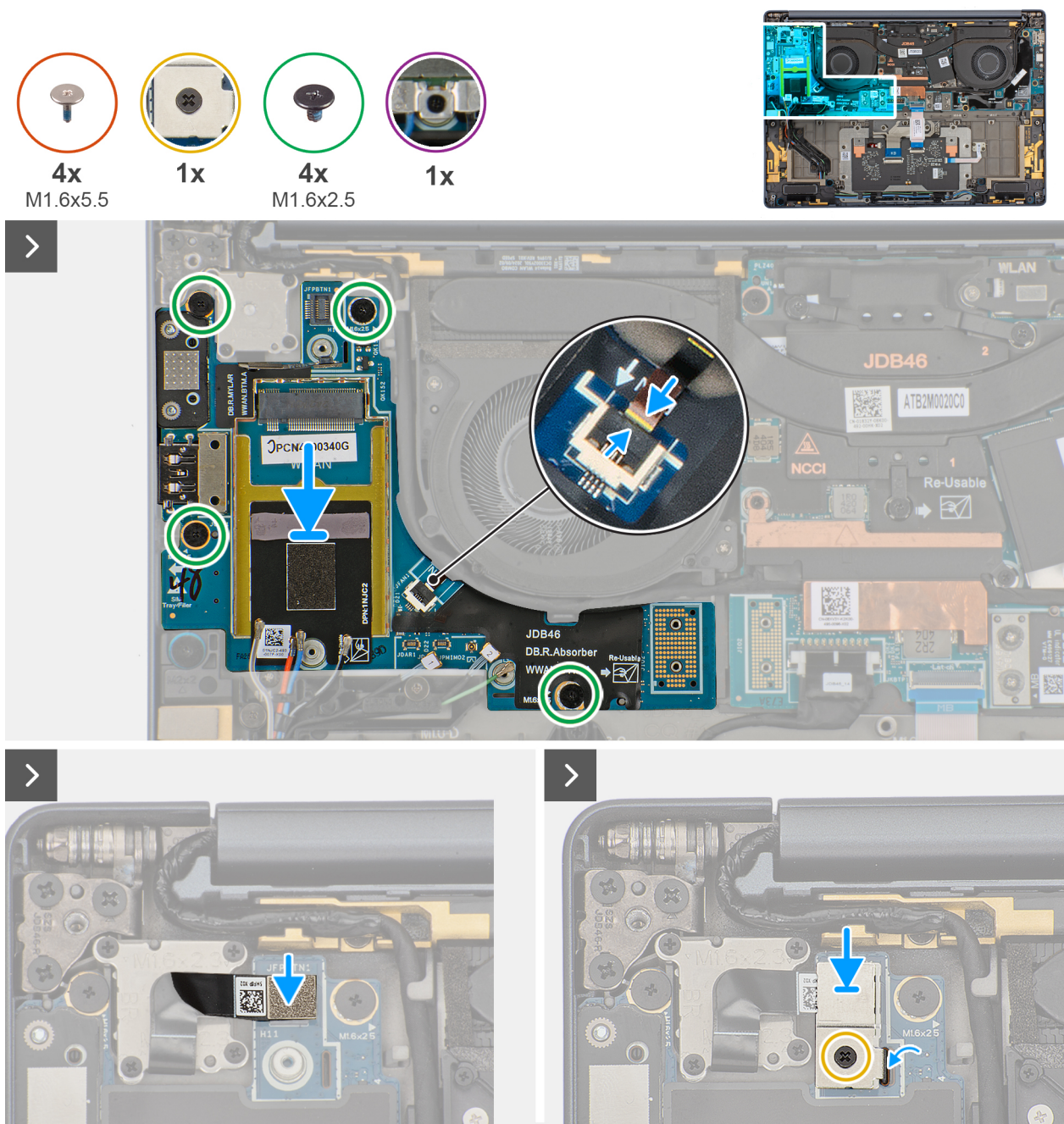
Figure 50. Installing the screws
