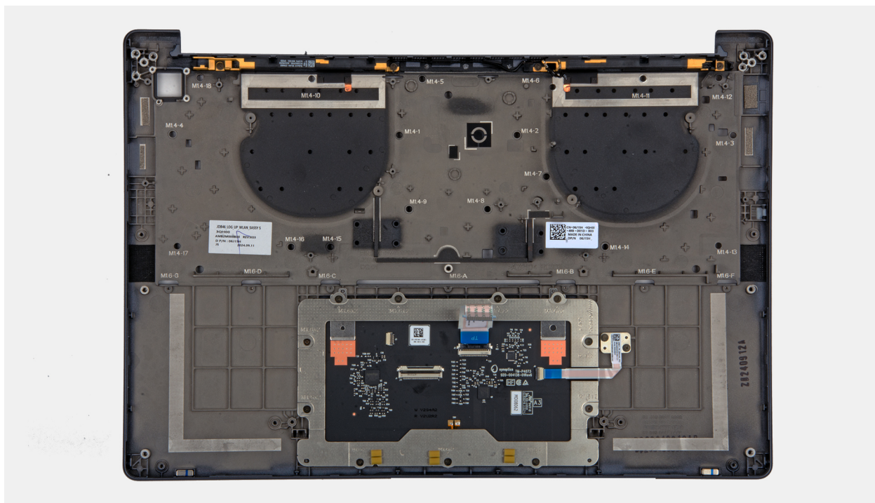
Figure 77. Palm-rest
