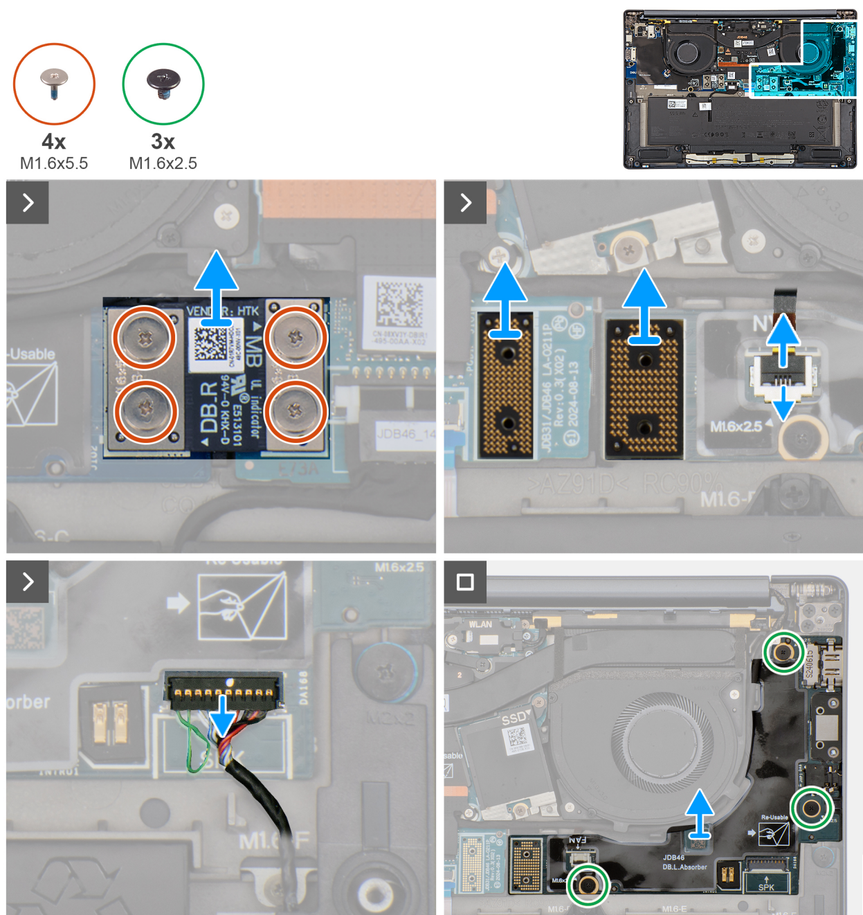
Figure 37. Removing the left I/O-board
