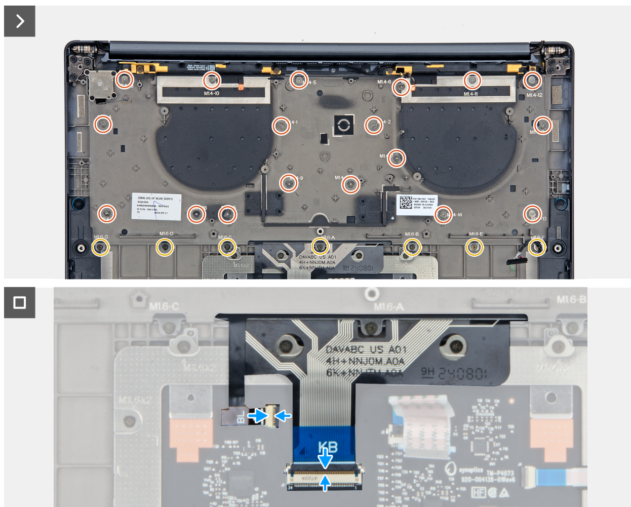
Figure 75. Installing the keyboard assembly
