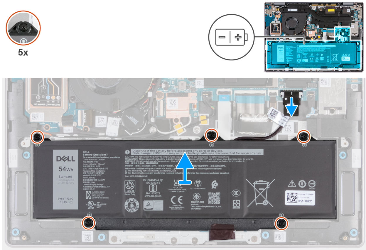
Figure 39. Removing the battery
