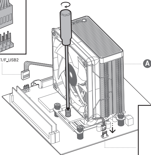
4-PIN/CPU_FAN/CPU_OPT
