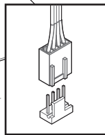
4-PIN/CPU_FAN/CPU_OPT
