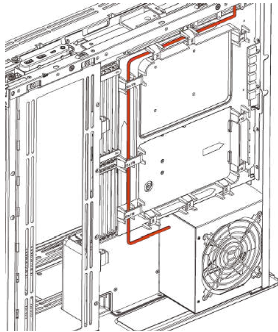
2 4+4-pin cable channel
