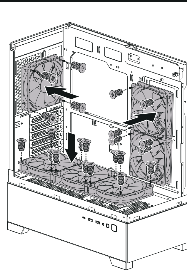
▼ Fan and Cooling System Setup
