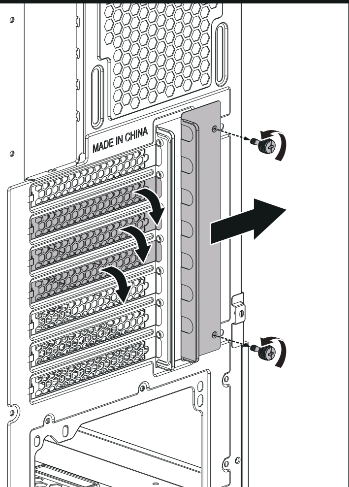
▼ GPU Installation
