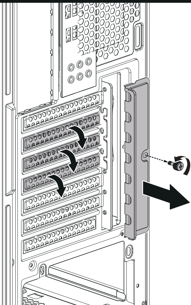
▼ GPU Installation
