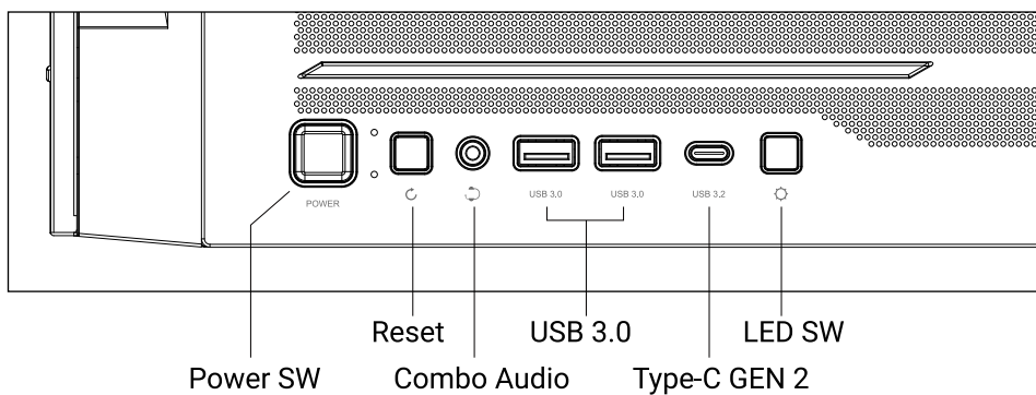
Power SW
