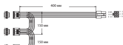
Peripheral IDE Power Connector
