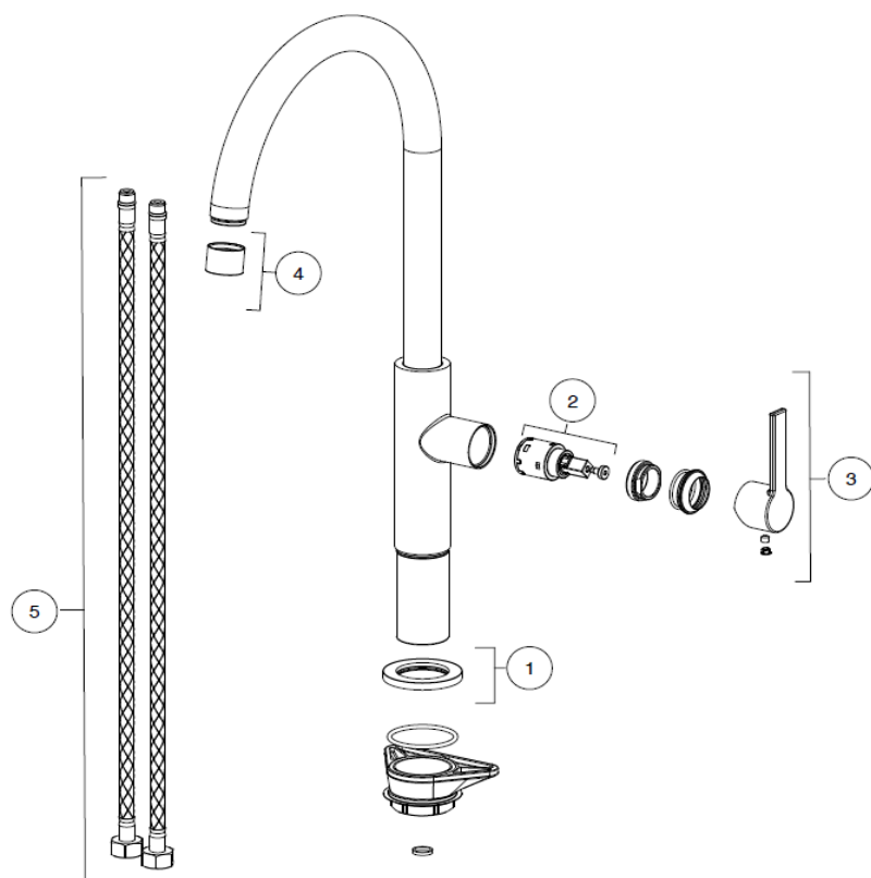
Tap Maris Slim J Swivel side HP CHR 115.0728.384
