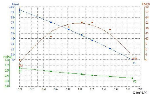
4QGD-1000
