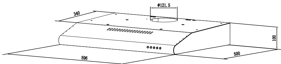
PL 6244 LED
